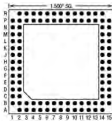
100 Pins – Footprint #15030
