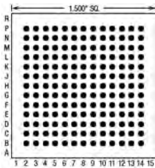
169 Pins – Footprint #15036
