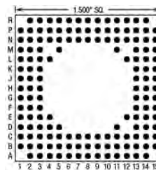
149 Pins – Footprint #15019
