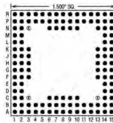
125 Pins – Footprint #15039
