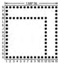
77 Pins – Footprint #15037
