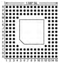
148 Pins – Footprint #15021
