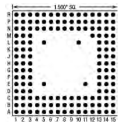
149 Pins – Footprint #15020
