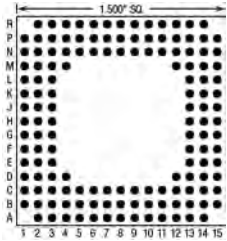
144 Pins – Footprint #15048
