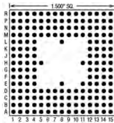
181 Pins – Footprint #15033
