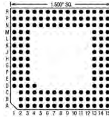
142 Pins – Footprint #15027
