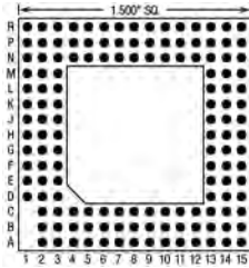
141 Pins – Footprint #15028
