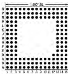
145 Pins – Footprint #15058
