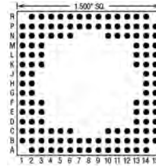
128 Pins – Footprint #15047
