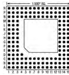
145 Pins – Footprint #15023
