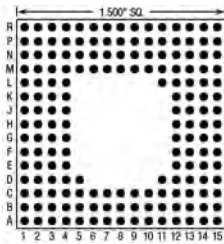
179 Pins – Footprint #15049
