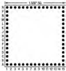
56 Pins – Footprint #15057
