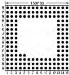
146 Pins – Footprint #15053
