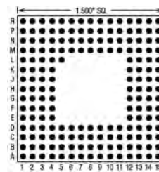
177 Pins – Footprint #15060
