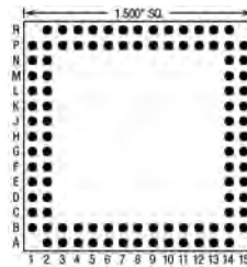
100 Pins – Footprint #15031
