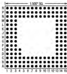
146 Pins – Footprint #15042
