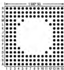
153 Pins – Footprint #15017
