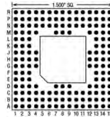
160 Pins – Footprint #15056
