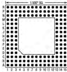
144 Pins – Footprint #15025
