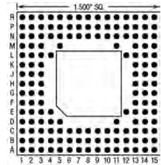
153 Pins – Footprint #15016
