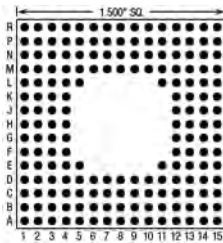
180 Pins – Footprint #15010
