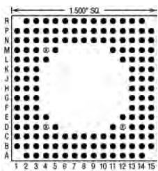
149 Pins – Footprint #15061
