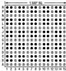
100 Pins – Footprint #15055
