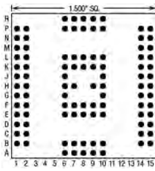
100 Pins – Footprint #15041
