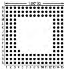
145 Pins – Footprint #15024
