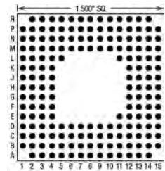
179 Pins – Footprint #15012
