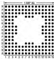
160 Pins – Footprint #15050
