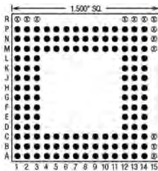
132 Pins – Footprint #15079
