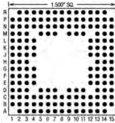
164 Pins – Footprint #15045
