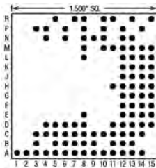
104 Pins – Footprint #15078
