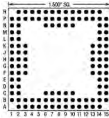
120 Pins – Footprint #15046
