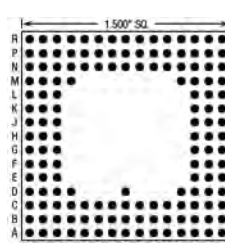
149 Pins – Footprint #15035
