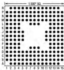
184 Pins – Footprint #15040
