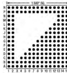
160 Pins – Footprint #15015
