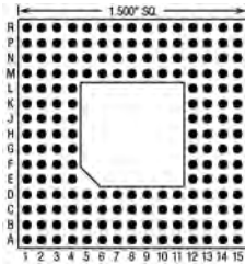
176 Pins – Footprint #15013
