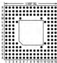
149 Pins – Footprint #15018
