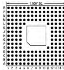
179 Pins – Footprint #15011
