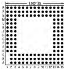
141 Pins – Footprint #15029
