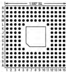
180 Pins – Footprint #15009
