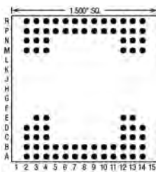
80 Pins – Footprint #15059
