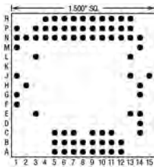
75 Pins – Footprint #15032
