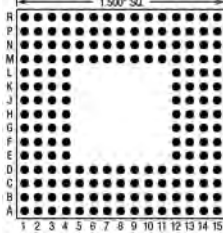
176 Pins – Footprint #15014
