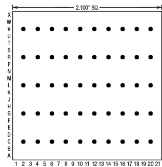
50 Pins – Footprint #21025
