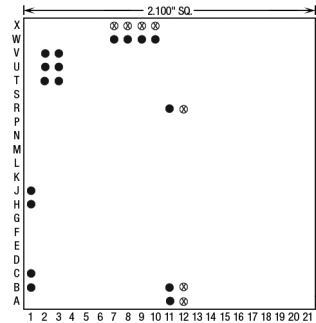
17 Pins – Footprint #21009
