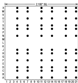
72 Pins – Footprint #21026
