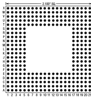
319 Pins – Footprint #21002
