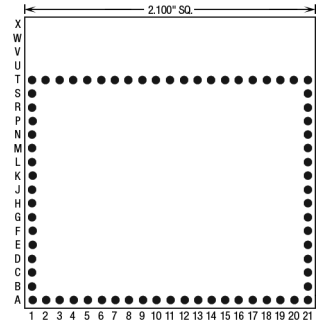
72 Pins – Footprint #21003
