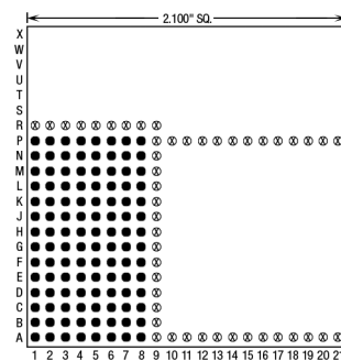
112 Pins – Footprint #21028
