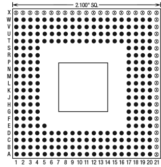
257 Pins – Footprint #21019
