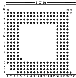
236 Pins – Footprint #21006
