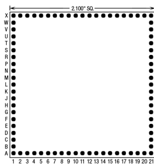
80 Pins – Footprint #21027
