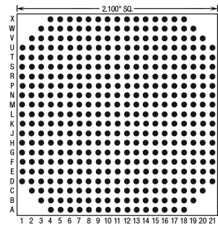
336 Pins – Footprint #21022
