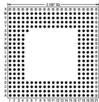
257 Pins – Footprint #21015
