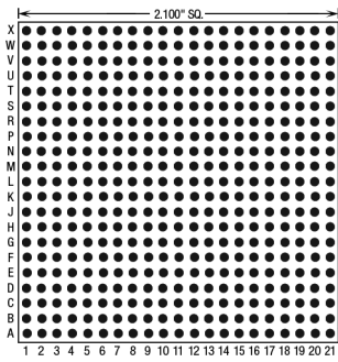
441 Pins – Footprint #21001
