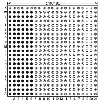
120 Pins – Footprint #21012
