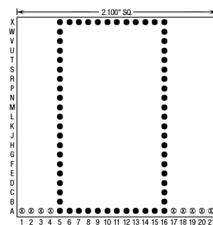
62 Pins – Footprint #21031
