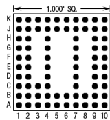
77 Pins – Footprint #10015
