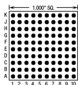
100 Pins – Footprint #10001
