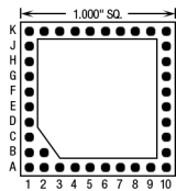
37 Pins – Footprint #10013
