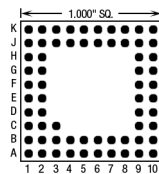
65 Pins – Footprint #10008
