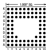
72 Pins – Footprint #10004
