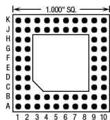
64 Pins – Footprint #10009
