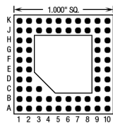
65 Pins – Footprint #10007
