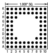
68 Pins – Footprint #10006
