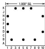
11 Pins – Footprint #10011
