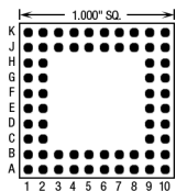
64 Pins – Footprint #10010
