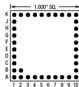
37 Pins – Footprint #10012
