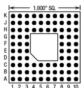
84 Pins – Footprint #10002
