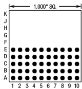
50 Pins – Footprint #10014
