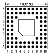
68 Pins – Footprint #10005
