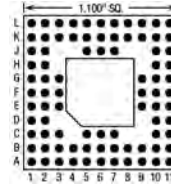
85 Pins – Footprint #11007
