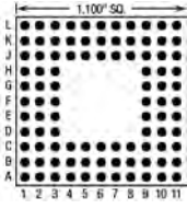
96 Pins – Footprint #11006
