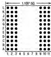
66 Pins – Footprint #11054
