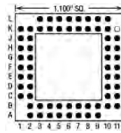
64 Pins – Footprint #11039
