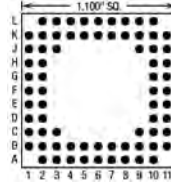
72 Pins – Footprint #11026
