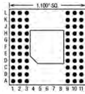
66 Pins – Footprint #11049
