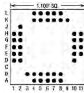
44 Pins – Footprint #11042
