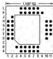
44 Pins – Footprint #11041
