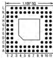
73 Pins – Footprint #11021
