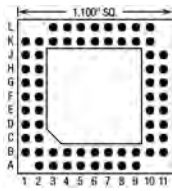
65 Pins – Footprint #11036
