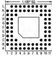
72 Pins – Footprint #11025
