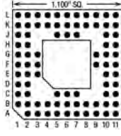
83 Pins – Footprint #11013
