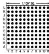
120 Pins – Footprint #11002
