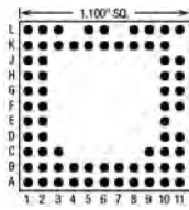
70 Pins – Footprint #11029
