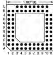
67 Pins – Footprint #11034
