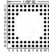
75 Pins – Footprint #11016
