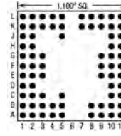
73 Pins – Footprint #11020
