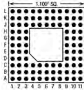
96 Pins – Footprint #11005
