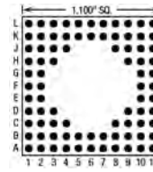
84 Pins – Footprint #11012
