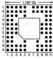
74 Pins – Footprint #11017
