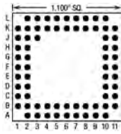
69 Pins – Footprint #11053
