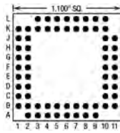
65 Pins – Footprint #11037
