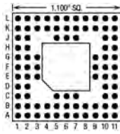
84 Pins – Footprint #11009
