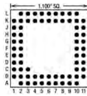
69 Pins – Footprint #11031
