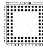
72 Pins – Footprint #11024
