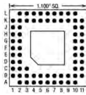
69 Pins – Footprint #11030
