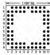
64 Pins – Footprint #11046
