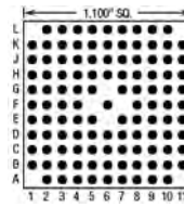
113 Pins – Footprint #11004
