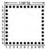
40 Pins – Footprint #11044
