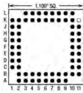
64 Pins – Footprint #11040
