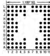
74 Pins – Footprint #11018
