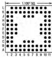
80 Pins – Footprint #11048
