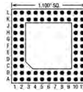
72 Pins – Footprint #11023
