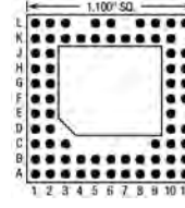
70 Pins – Footprint #11028
