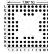
85 Pins – Footprint #11008
