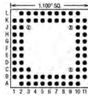
69 Pins – Footprint #11055
