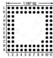
73 Pins – Footprint #11050
