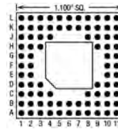
84 Pins – Footprint #11011
