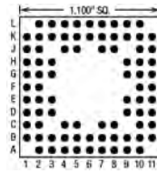
84 Pins – Footprint #11047
