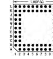
71 Pins – Footprint #11027
