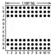
65 Pins – Footprint #11045
