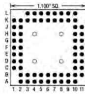
65 Pins – Footprint #11038
