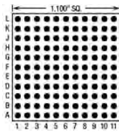
121 Pins – Footprint #11001
