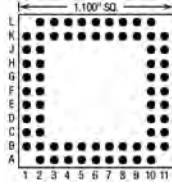
68 Pins – Footprint #11033
