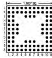
84 Pins – Footprint #11010
