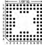
83 Pins – Footprint #11014
