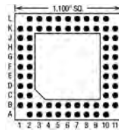
68 Pins – Footprint #11032
