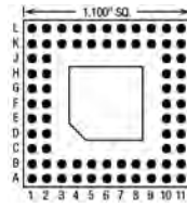
72 Pins – Footprint #11051
