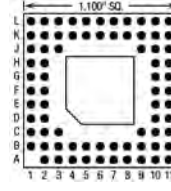
75 Pins – Footprint #11015
