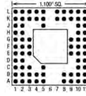
73 Pins – Footprint #11019
