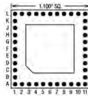
40 Pins – Footprint #11043
