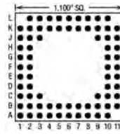
73 Pins – Footprint #11022
