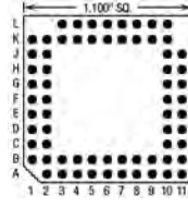
67 Pins – Footprint #11035
