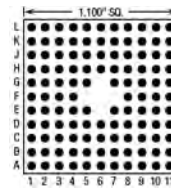
116 Pins – Footprint #11003
