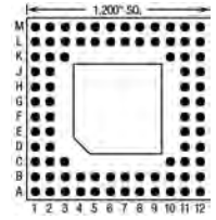
84 Pins – Footprint #12012
