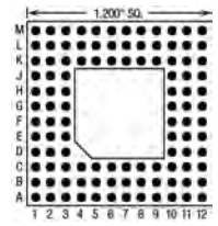
108 Pins – Footprint #12004
