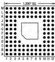
109 Pins – Footprint #12002
