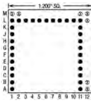
31 Pins – Footprint #12026
