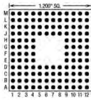
128 Pins – Footprint #12025
