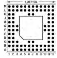
88 Pins – Footprint #12008
