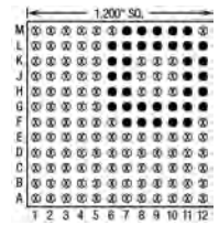
36 Pins – Footprint #12020
