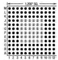
108 Pins – Footprint #12024
