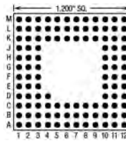
109 Pins – Footprint #12003
