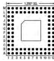
80 Pins – Footprint #12027
