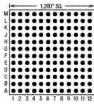
144 Pins – Footprint #12001
