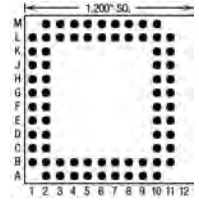
72 Pins – Footprint #12016
