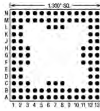
101 Pins – Footprint #13023
