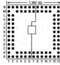
84 Pins – Footprint #13056
