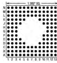
133 Pins – Footprint #13052
