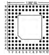
100 Pins – Footprint #13024
