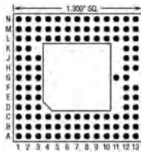
112 Pins – Footprint #13122
