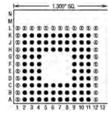
84 Pins – Footprint #13125
