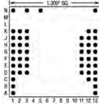
52 Pins – Footprint #13037
