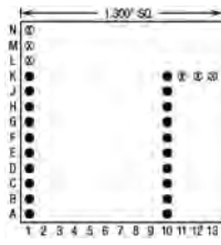
20 Pins – Footprint #13098
