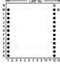
24 Pins – Footprint #13096
