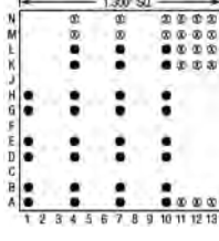
30 Pins – Footprint #13115
