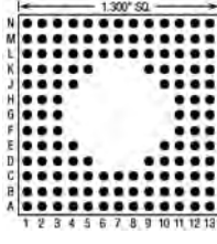
132 Pins – Footprint #13038
