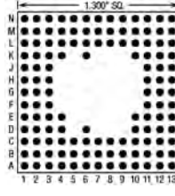
128 Pins – Footprint #13039
