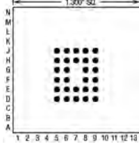
28 Pins – Footprint #13094
