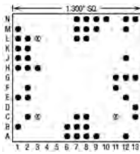
45 Pins – Footprint #13107
