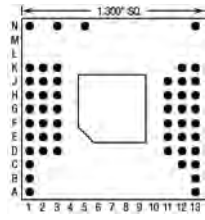
52 Pins – Footprint #13036
