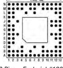
88 Pins – Footprint #13049
