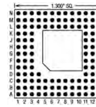
121 Pins – Footprint #13012
