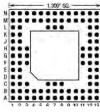
101 Pins – Footprint #13022
