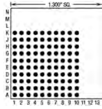
100 Pins – Footprint #13105
