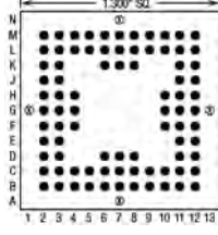
84 Pins – Footprint #13066
