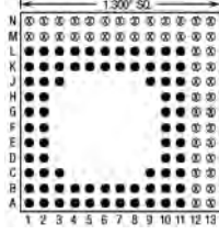
76 Pins – Footprint #13110
