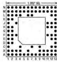
85 Pins – Footprint #13060
