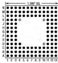
121 Pins – Footprint #13106
