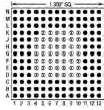
121 Pins – Footprint #13121
