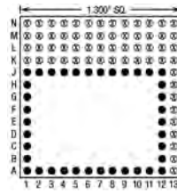
38 Pins – Footprint #13133
