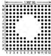
133 Pins – Footprint #13055
