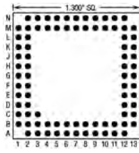
85 Pins – Footprint #13033
