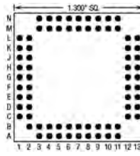
73 Pins – Footprint #13035
