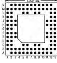
100 Pins – Footprint #13114
