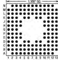
132 Pins – Footprint #13072
