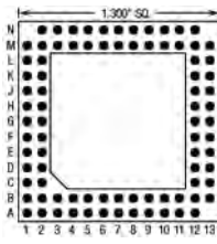
85 Pins – Footprint #13030
