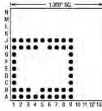
44 Pins – Footprint #13104
