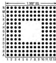
144 Pins – Footprint #13003
