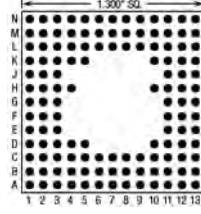
128 Pins – Footprint #13064
