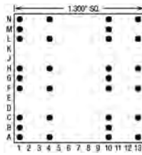
30 Pins – Footprint #13108
