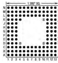
121 Pins – Footprint #13077
