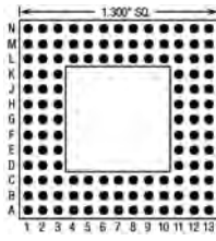
119 Pins – Footprint #13018
