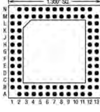
84 Pins – Footprint #13042
