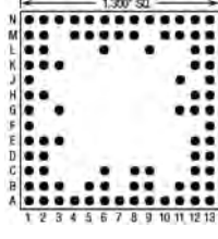
93 Pins – Footprint #13041
