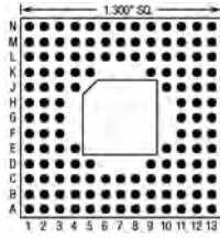
132 Pins – Footprint #13102
