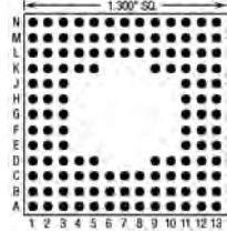
128 Pins – Footprint #13093
