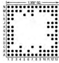
86 Pins – Footprint #13057
