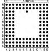
114 Pins – Footprint #13062
