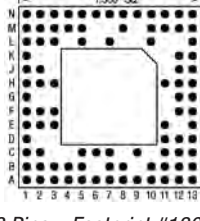
93 Pins – Footprint #13045
