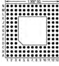
120 Pins – Footprint #13014
