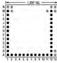
34 Pins – Footprint #13128
