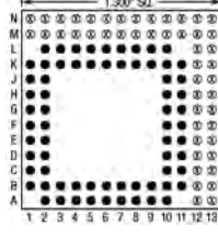
68 Pins – Footprint #13116
