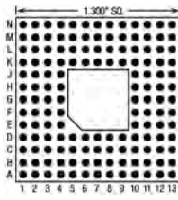
144 Pins – Footprint #13002
