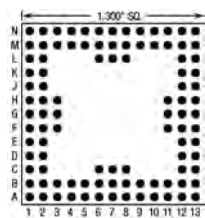
100 Pins – Footprint #13061
