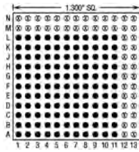
121 Pins – Footprint #13131
