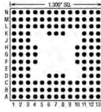
132 Pins – Footprint #13007
