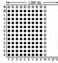
108 Pins – Footprint #13129
