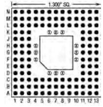
120 Pins – Footprint #13130
