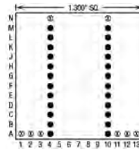
24 Pins – Footprint #13137
