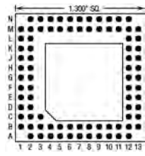
85 Pins – Footprint #13032
