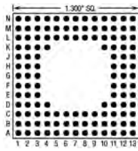
124 Pins – Footprint #13009
