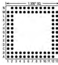
85 Pins – Footprint #13031
