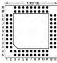
73 Pins – Footprint #13034
