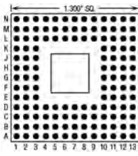
133 Pins – Footprint #13004
