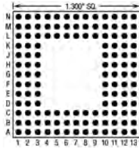
133 Pins – Footprint #13005
