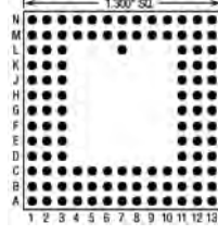
114 Pins – Footprint #13068
