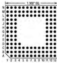
120 Pins – Footprint #13017
