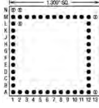
44 Pins – Footprint #13090
