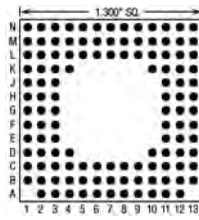
122 Pins – Footprint #13011
