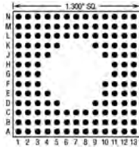
133 Pins – Footprint #13054
