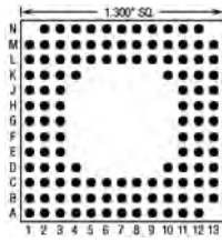
121 Pins – Footprint #13058
