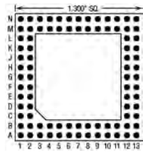
88 Pins – Footprint #13028
