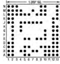
90 Pins – Footprint #13089
