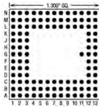
114 Pins – Footprint #13021
