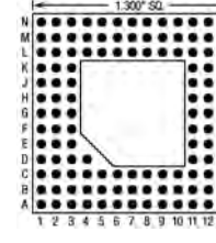
120 Pins – Footprint #13016
