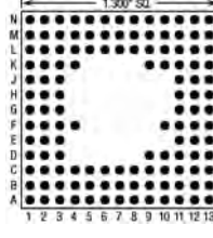
128 Pins – Footprint #13043
