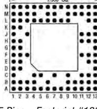
95 Pins – Footprint #13047
