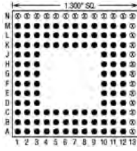
108 Pins – Footprint #13119
