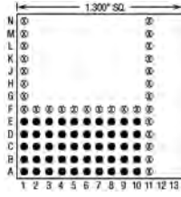
50 Pins – Footprint #13118
