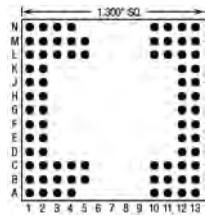
80 Pins – Footprint #13109
