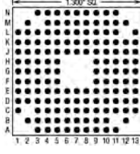
144 Pins – Footprint #13095
