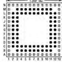
68 Pins – Footprint #13117
