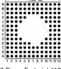
133 Pins – Footprint #13046
