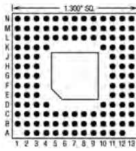
122 Pins – Footprint #13010
