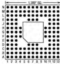
132 Pins – Footprint #13006
