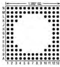
100 Pins – Footprint #13025
