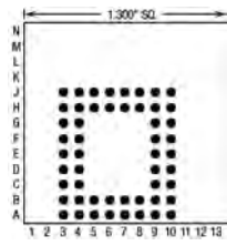
40 Pins – Footprint #13101
