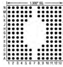
132 Pins – Footprint #13085
