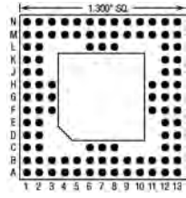
100 Pins – Footprint #13081
