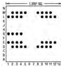
36 Pins – Footprint #13123
