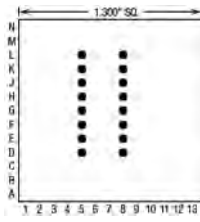
16 Pins – Footprint #13074
