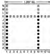
20 Pins – Footprint #13120
