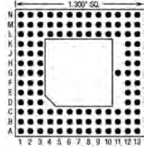
114 Pins – Footprint #13040
