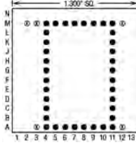
34 Pins – Footprint #13091
