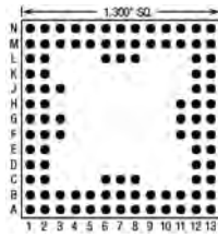
100 Pins – Footprint #13059
