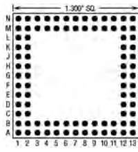
88 Pins – Footprint #13029
