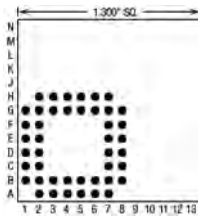
44 Pins – Footprint #13099
