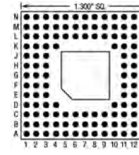
124 Pins – Footprint #13008
