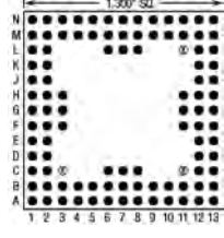
103 Pins – Footprint #13097
