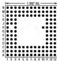
113 Pins – Footprint #13050
