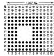
84 Pins – Footprint #13134
