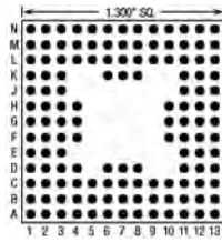
132 Pins – Footprint #13132
