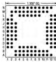
96 Pins – Footprint #13027
