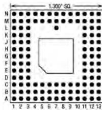
114 Pins – Footprint #13051
