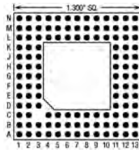
119 Pins – Footprint #13019
