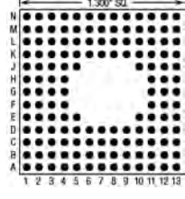
143 Pins – Footprint #13044
