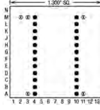
24 Pins – Footprint #13092
