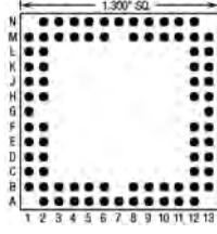
80 Pins – Footprint #13070
