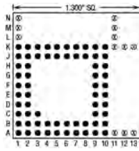
65 Pins – Footprint #13135
