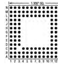
119 Pins – Footprint #13020
