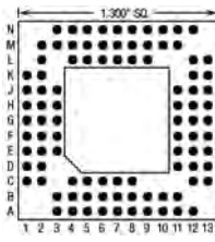
96 Pins – Footprint #13026
