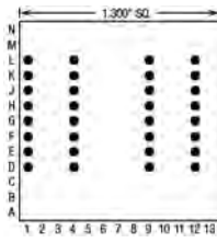
32 Pins – Footprint #13075
