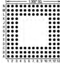
120 Pins – Footprint #13015
