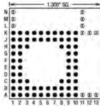
68 Pins – Footprint #13126
