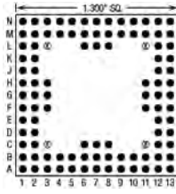
101 Pins – Footprint #13103
