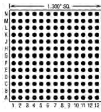
169 Pins – Footprint #13001
