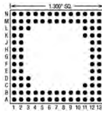
104 Pins – Footprint #13100
