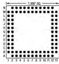
84 Pins – Footprint #13053
