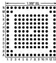
132 Pins – Footprint #13076
