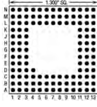
121 Pins – Footprint #13013
