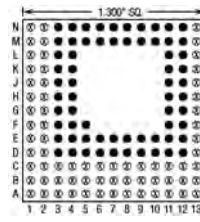
65 Pins – Footprint #13124
