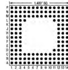
135 Pins – Footprint #14012
