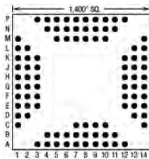
94 Pins – Footprint #14022
