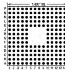
180 Pins – Footprint #14003
