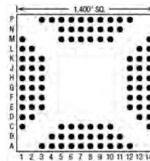
94 Pins – Footprint #14023
