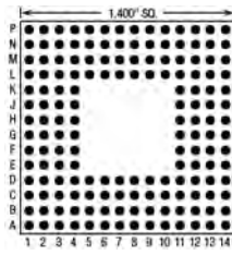
101 Pins – Footprint #14029
