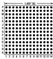
196 Pins – Footprint #14001
