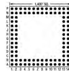
96 Pins – Footprint #14024
