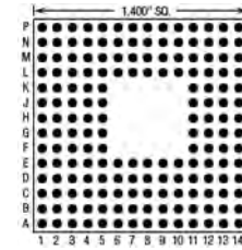
171 Pins – Footprint #14008
