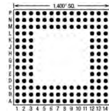
132 Pins – Footprint #14016
