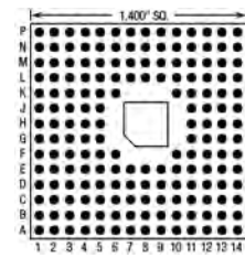
175 Pins – Footprint #14004
