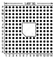
180 Pins – Footprint #14002
