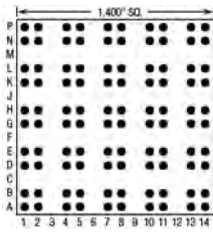
100 Pins – Footprint #14025
