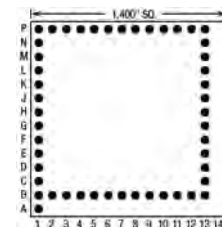
49 Pins – Footprint #14020
