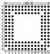
125 Pins – Footprint #14021
