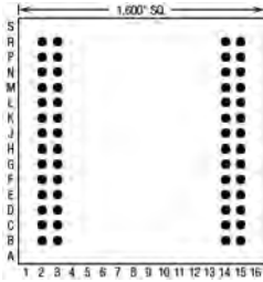
56 Pins – Footprint #16025
