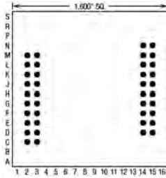
40 Pins – Footprint #16026
