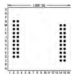
40 Pins – Footprint #16024
