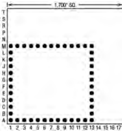
54 Pins – Footprint #17058
