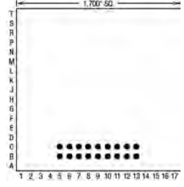
18 Pins – Footprint #17041
