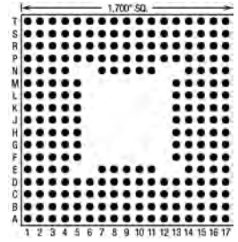
232 Pins – Footprint #17037
