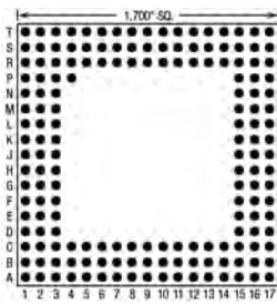
169 Pins – Footprint #17002
