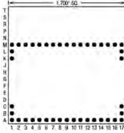
43 Pins – Footprint #17019
