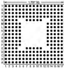
228 Pins – Footprint #17036
