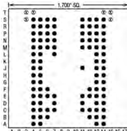
100 Pins – Footprint #17049
