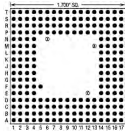
209 Pins – Footprint #17057
