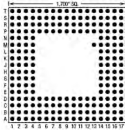
209 Pins – Footprint #17030
