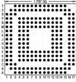
208 Pins – Footprint #17039
