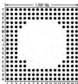
181 Pins – Footprint #17015
