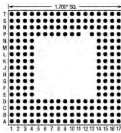
207 Pins – Footprint #17045
