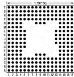
225 Pins – Footprint #17008
