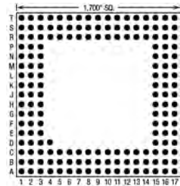
169 Pins – Footprint #17012
