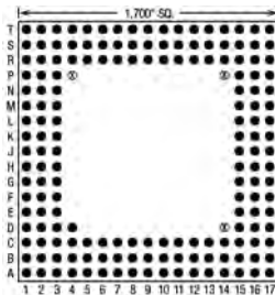
169 Pins – Footprint #17053
