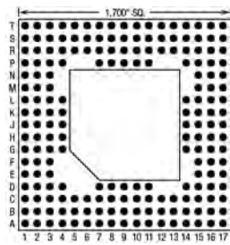
192 Pins – Footprint #17043
