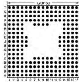
226 Pins – Footprint #17060
