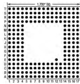
209 Pins – Footprint #17046
