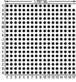
288 Pins – Footprint #17040
