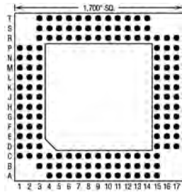
144 Pins – Footprint #17005
