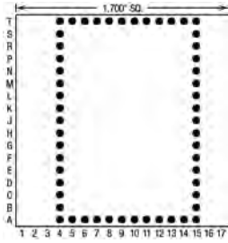
34 Pins – Footprint #17034
