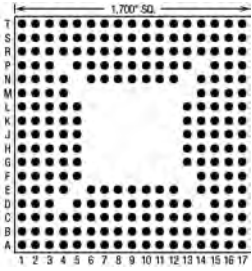
54 Pins – Footprint #17035
