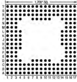
192 Pins – Footprint #17025
