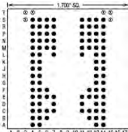
100 Pins – Footprint #17048
