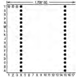
240 Pins – Footprint #17033
