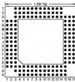
145 Pins – Footprint #17003
