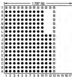
180 Pins – Footprint #17052
