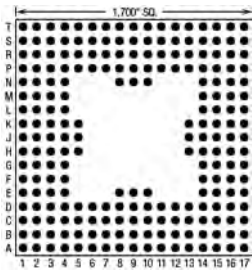
216 Pins – Footprint #17023
