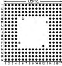
209 Pins – Footprint #17018
