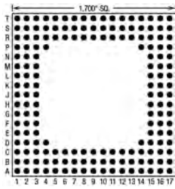
172 Pins – Footprint #17021
