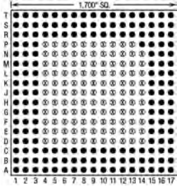
169 Pins – Footprint #17026
