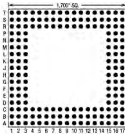
168 Pins – Footprint #17011
