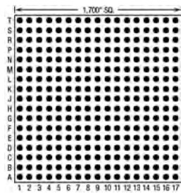
289 Pins – Footprint #17001
