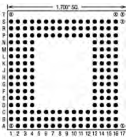
175 Pins – Footprint #17044
