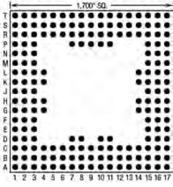
185 Pins – Footprint #17031
