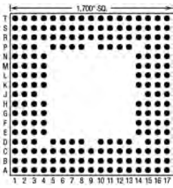
196 Pins – Footprint #17022
