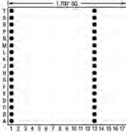
34 Pins – Footprint #17028
