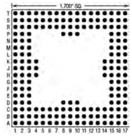
180 Pins – Footprint #17024
