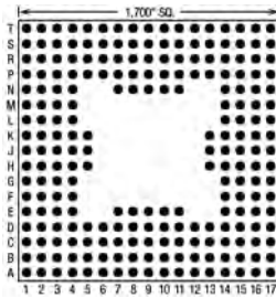
225 Pins – Footprint #17007
