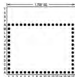
54 Pins – Footprint #17016
