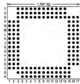
145 Pins – Footprint #17004
