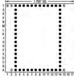
54 Pins – Footprint #17038
