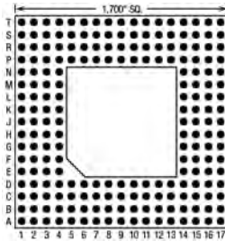
208 Pins – Footprint #17059
