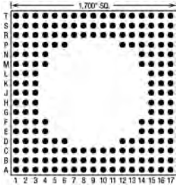
188 Pins – Footprint #17032
