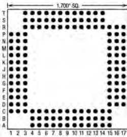
144 Pins – Footprint #17006
