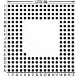
209 Pins – Footprint #17020
