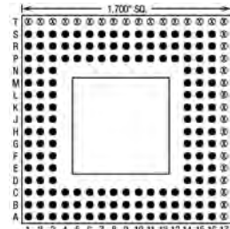
156 Pins – Footprint #17050
