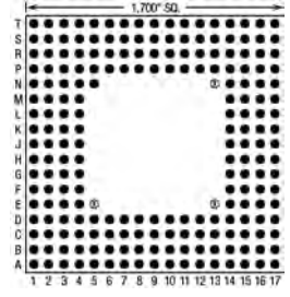
209 Pins – Footprint #17029
