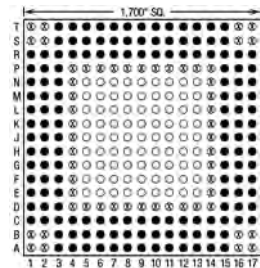
104 Pins – Footprint #17054
