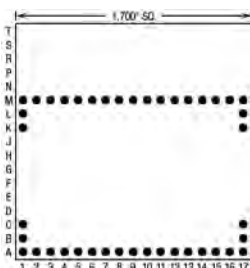
43 Pins – Footprint #17014
