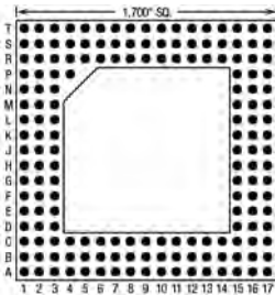
169 Pins – Footprint #17010
