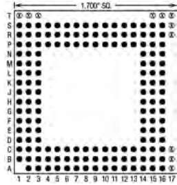
155 Pins – Footprint #17061
