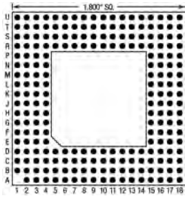
223 Pins – Footprint #18039
