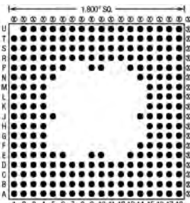
241 Pins – Footprint #18025-ZIF
