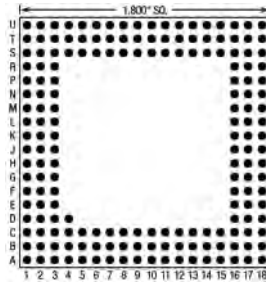
181 Pins – Footprint #18041
