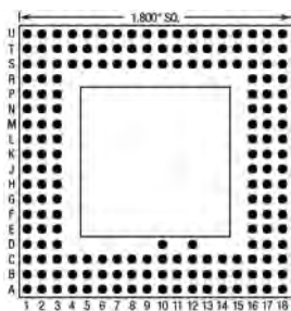
182 Pins – Footprint #18022
