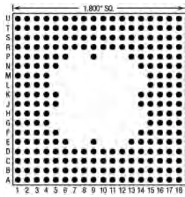
246 Pins – Footprint #18034
