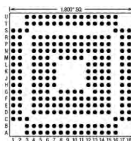
240 Pins – Footprint #18033
