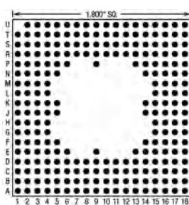
241 Pins – Footprint #18027
