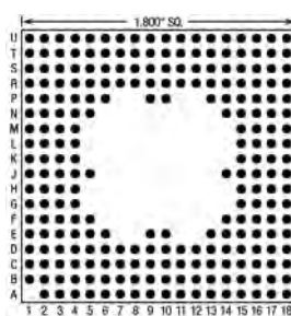
241 Pins – Footprint #18028
