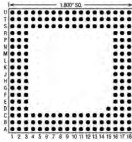
181 Pins – Footprint #18040
