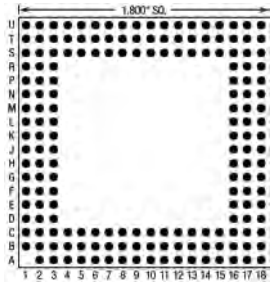
179 Pins – Footprint #18038
