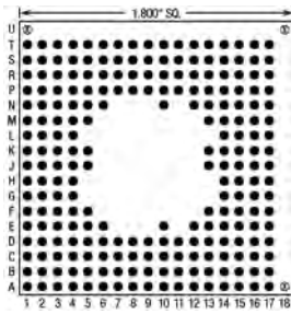
242 Pins – Footprint #18036
