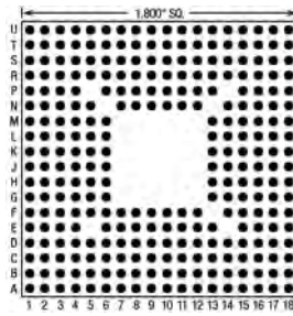
281 Pins – Footprint #18037
