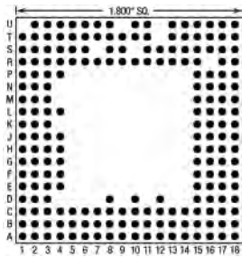
206 Pins – Footprint #18031
