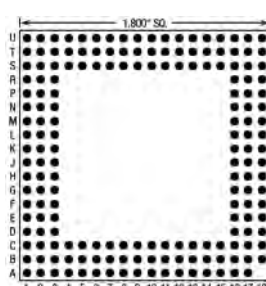
179 Pins – Footprint #18024
