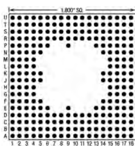
242 Pins – Footprint #18026
