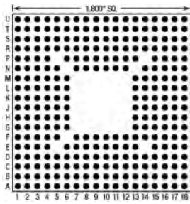
281 Pins – Footprint #18035
