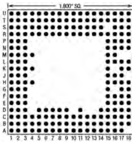
206 Pins – Footprint #18042
