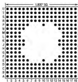
241 Pins – Footprint #18021
