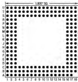
179 Pins – Footprint #18030
