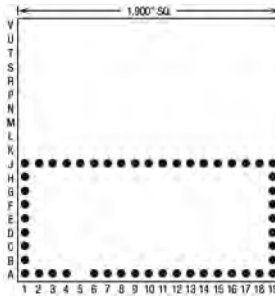
51 Pins – Footprint #19018
