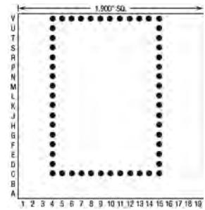
54 Pins – Footprint #19016
