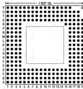
236 Pins – Footprint #19009
