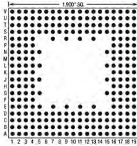
257 Pins – Footprint #19020
