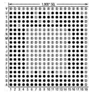
206 Pins – Footprint #19046
