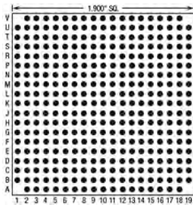
357 Pins – Footprint #19026
