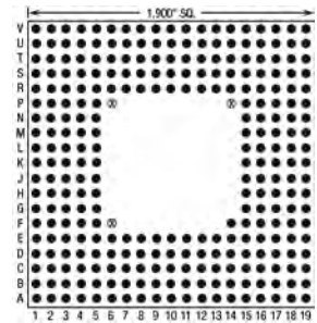
281 Pins – Footprint #19028
