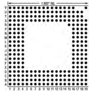
237 Pins – Footprint #19019
