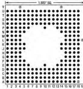
241 Pins – Footprint #19021
