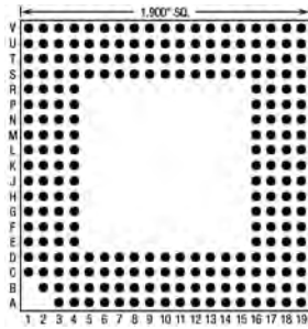
238 Pins – Footprint #19004
