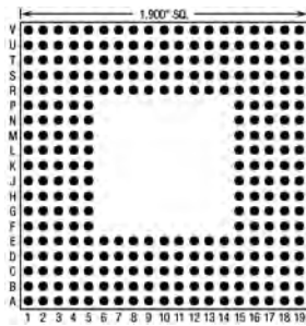
280 Pins – Footprint #19006
