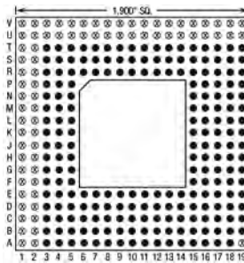
280 Pins – Footprint #19024
