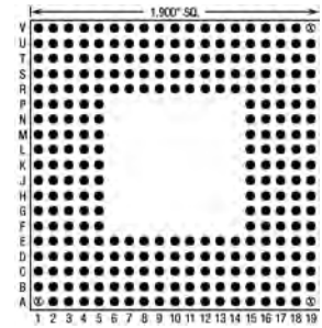
277 Pins – Footprint #19005
