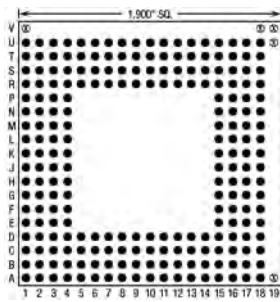
224 Pins – Footprint #19044
