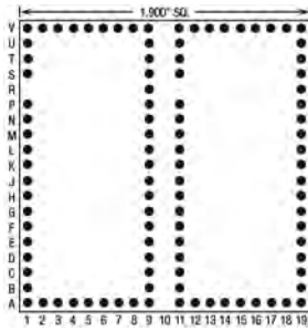
102 Pins – Footprint #19017
