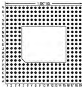
262 Pins – Footprint #19014
