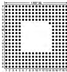
281 Pins – Footprint #19012
