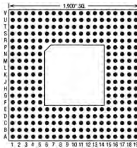
280 Pins – Footprint #19027
