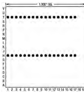
34 Pins – Footprint #19002
