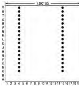
34 Pins – Footprint #19015
