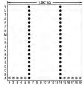
39 Pins – Footprint #19022
