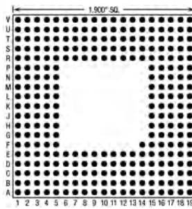
281 Pins – Footprint #19045
