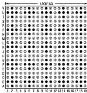
125 Pins – Footprint #19023
