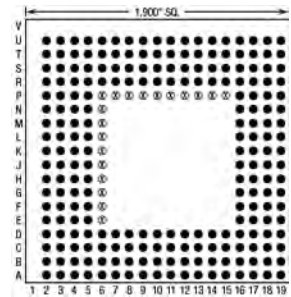
224 Pins – Footprint #19025
