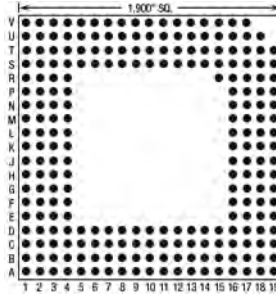
238 Pins – Footprint #19007
