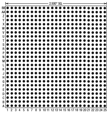
625 Pins – Footprint #25001
