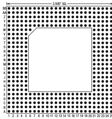
401 Pins – Footprint #25002
