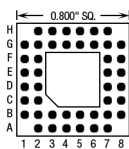
44 Pins – Footprint #08002
