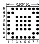
45 Pins – Footprint #08007
