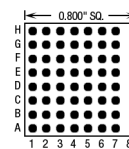
56 Pins – Footprint #08004
