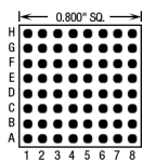
64 Pins – Footprint #08001
