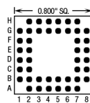
44 Pins – Footprint #08003
