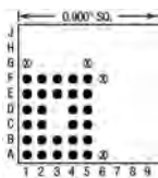
28 Pins – Footprint #09029
