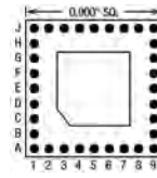
32 Pins – Footprint #09016
