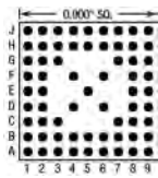
65 Pins – Footprint #09005
