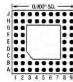
56 Pins – Footprint #09008
