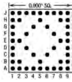
48 Pins – Footprint #09013
