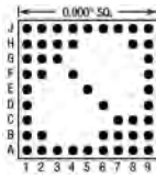
49 Pins – Footprint #09014
