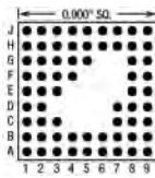
65 Pins – Footprint #09006
