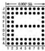
57 Pins – Footprint #09007
