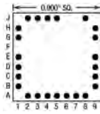
24 Pins – Footprint #09023
