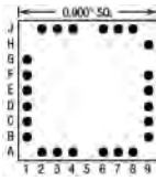
24 Pins – Footprint #09022
