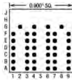
40 Pins – Footprint #09015
