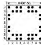
32 Pins – Footprint #09024
