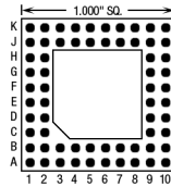
64 Pins – Footprint #10009
