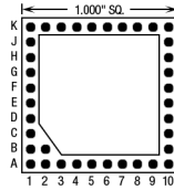
37 Pins – Footprint #10013
