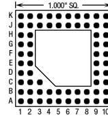
65 Pins – Footprint #10007
