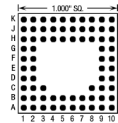
72 Pins – Footprint #10004
