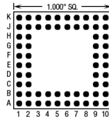
64 Pins – Footprint #10010
