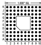
84 Pins – Footprint #10002
