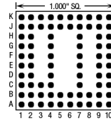
77 Pins – Footprint #10015
