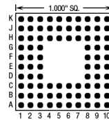
84 Pins – Footprint #10003
