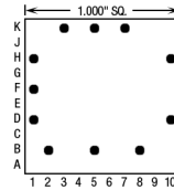
11 Pins – Footprint #10011
