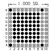
59 Pins – Footprint #10016
