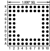
65 Pins – Footprint #10008
