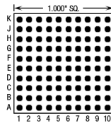
100 Pins – Footprint #10001
