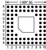
68 Pins – Footprint #10005
