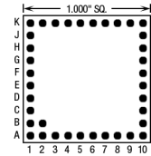
37 Pins – Footprint #10012
