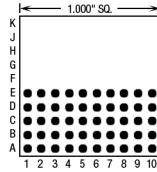
50 Pins – Footprint #10014
