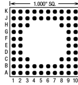
68 Pins – Footprint #10006
