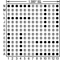
48 Pins – Footprint #13113
