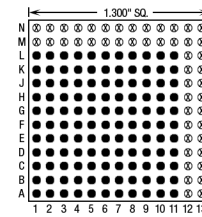
121 Pins – Footprint #13131
