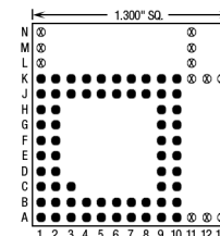
65 Pins – Footprint #13135
