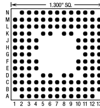
132 Pins – Footprint #13072
