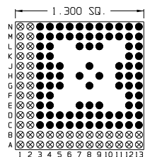
88 Pins – Footprint #13147
