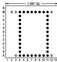
34 Pins – Footprint #13091
