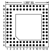
85 Pins – Footprint #13032
