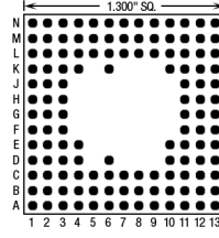
128 Pins – Footprint #13039
