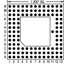
114 Pins – Footprint #13040
