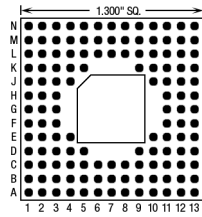
132 Pins – Footprint #13102
