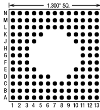
133 Pins – Footprint #13055
