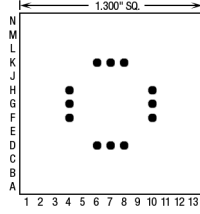
12 Pins – Footprint #13111
