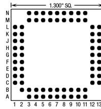
73 Pins – Footprint #13035
