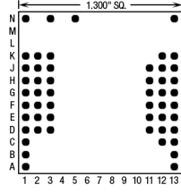
52 Pins – Footprint #13037
