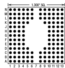
132 Pins – Footprint #13085
