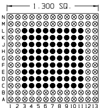
81 Pins – Footprint #13146
