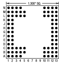
80 Pins – Footprint #13109
