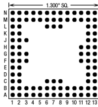
100 Pins – Footprint #13059
