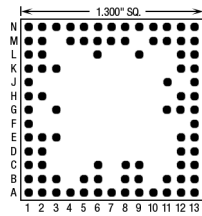
93 Pins – Footprint #13041
