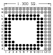
69 Pins – Footprint #13142
