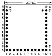
34 Pins – Footprint #13128
