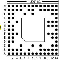
88 Pins – Footprint #13048
