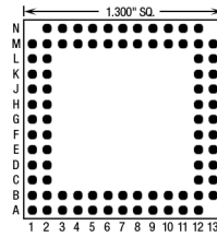
85 Pins – Footprint #13031
