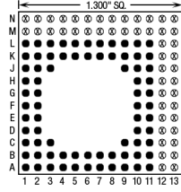
76 Pins – Footprint #13110
