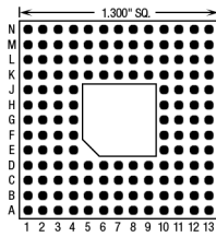
144 Pins – Footprint #13002
