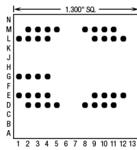
36 Pins – Footprint #13123
