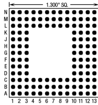
133 Pins – Footprint #13005
