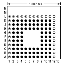
84 Pins – Footprint #13125
