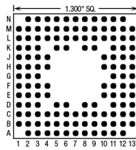
132 Pins – Footprint #13079
