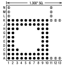
68 Pins – Footprint #13126
