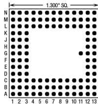
114 Pins – Footprint #13021
