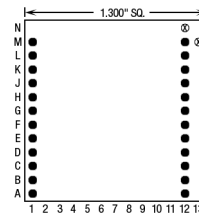
24 Pins – Footprint #13096
