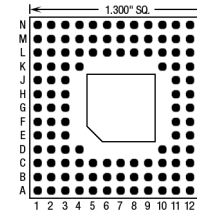
124 Pins – Footprint #13008
