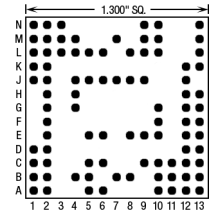
90 Pins – Footprint #13089
