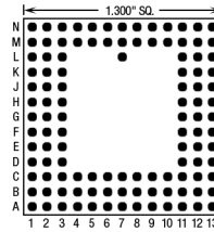
114 Pins – Footprint #13068
