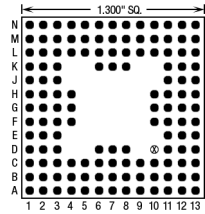
132 Pins – Footprint #13073
