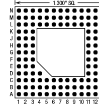
121 Pins – Footprint #13016
