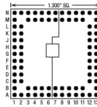
84 Pins – Footprint #13056
