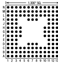
132 Pins – Footprint #13007
