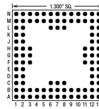
101 Pins – Footprint #13080
