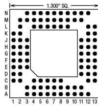
96 Pins – Footprint #13026
