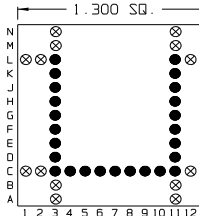
25 Pins – Footprint #13145
