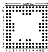
100 Pins – Footprint #13082
