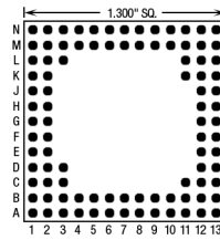
104 Pins – Footprint #13100
