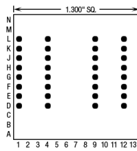
32 Pins – Footprint #13075
