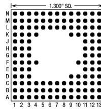
128 Pins – Footprint #13043
