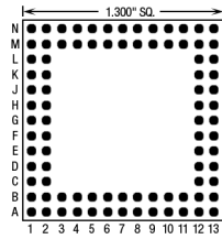
88 Pins – Footprint #13029
