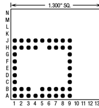
44 Pins – Footprint #13104
