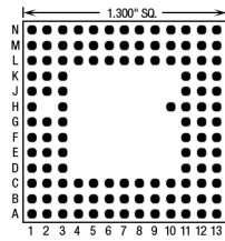
113 Pins – Footprint #13050
