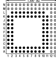
68 Pins – Footprint #13116
