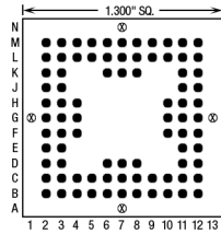
84 Pins – Footprint #13066
