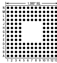
144 Pins – Footprint #13003
