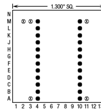
24 Pins – Footprint #13092
