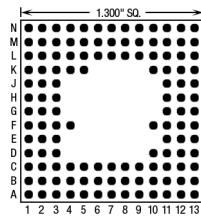
128 Pins – Footprint #13078
