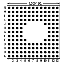
143 Pins – Footprint #13044
