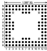
101 Pins – Footprint #13103
