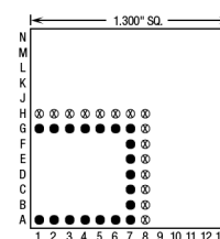
19 Pins – Footprint #13136
