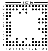
86 Pins – Footprint #13057
