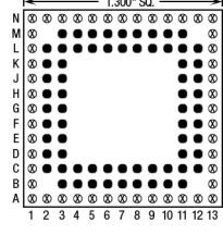
68 Pins – Footprint #13117
