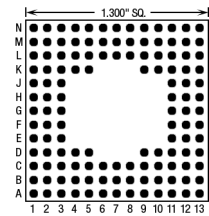
128 Pins – Footprint #13093
