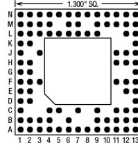
95 Pins – Footprint #13047
