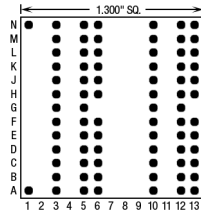
78 Pins – Footprint #13086
