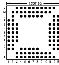
96 Pins – Footprint #13027
