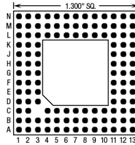
119 Pins – Footprint #13019
