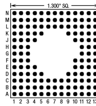
133 Pins – Footprint #13052
