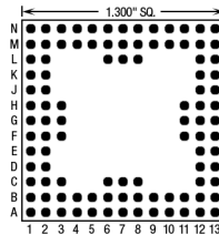
101 Pins – Footprint #13023
