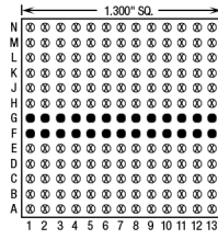
26 Pins – Footprint #13087
