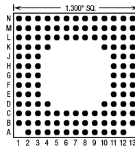
122 Pins – Footprint #13011
