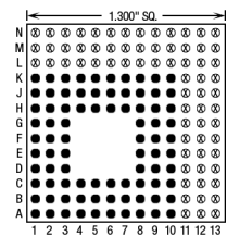
84 Pins – Footprint #13134
