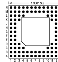
100 Pins – Footprint #13024
