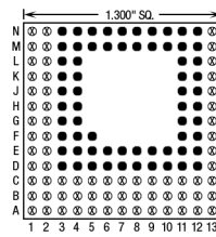
65 Pins – Footprint #13124
