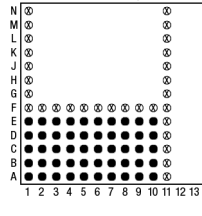
50 Pins – Footprint #13118
