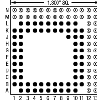
69 Pins – Footprint #13112
