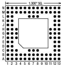
101 Pins – Footprint #13022
