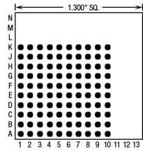
100 Pins – Footprint #13105
