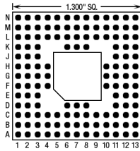
132 Pins – Footprint #13006
