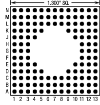
132 Pins – Footprint #13065
