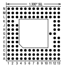
112 Pins – Footprint #13122
