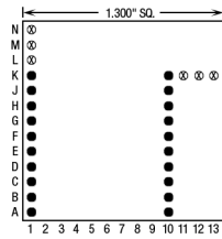
20 Pins – Footprint #13098
