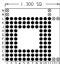
96 Pins – Footprint #13148
