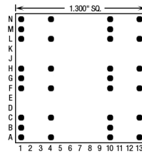
30 Pins – Footprint #13108
