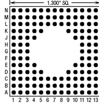
132 Pins – Footprint #13038
