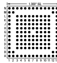
132 Pins – Footprint #13076
