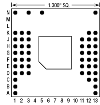
52 Pins – Footprint #13036
