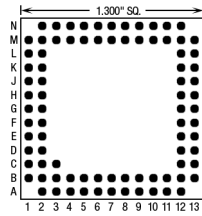
85 Pins – Footprint #13033
