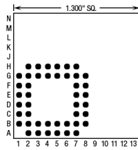
44 Pins – Footprint #13099
