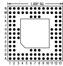
100 Pins – Footprint #13081
