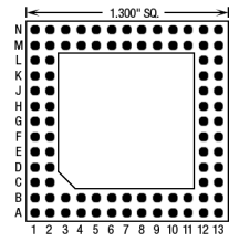
88 Pins – Footprint #13028
