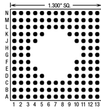
133 Pins – Footprint #13054
