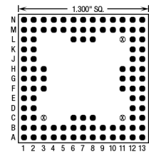
103 Pins – Footprint #13097
