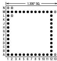
44 Pins – Footprint #13090
