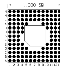
136 Pins – Footprint #13150
