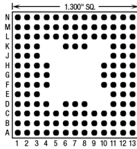
133 Pins – Footprint #13067
