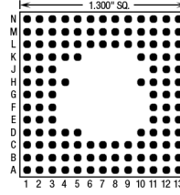
128 Pins – Footprint #13064
