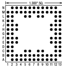
100 Pins – Footprint #13071
