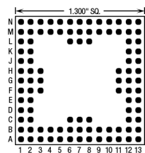
100 Pins – Footprint #13061
