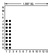
18 Pins – Footprint #13083
