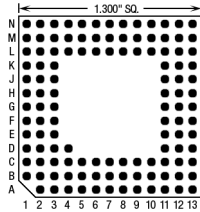
120 Pins – Footprint #13017
