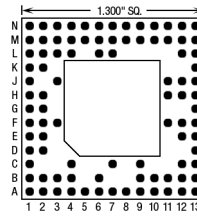
85 Pins – Footprint #13060
