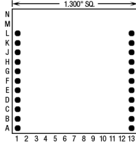
22 Pins – Footprint #13063
