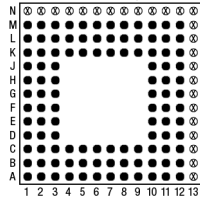
108 Pins – Footprint #13119
