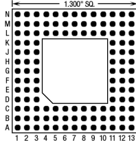
120 Pins – Footprint #13014
