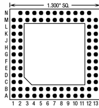
85 Pins – Footprint #13030
