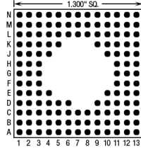
133 Pins – Footprint #13046
