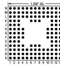
132 Pins – Footprint #13132
