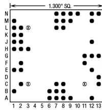
45 Pins – Footprint #13107
