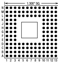
133 Pins – Footprint #13004
