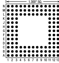
120 Pins – Footprint #13015
