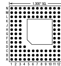
121 Pins – Footprint #13012
