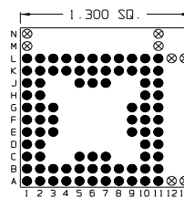
84 Pins – Footprint #13139
