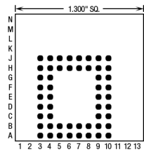
40 Pins – Footprint #13101
