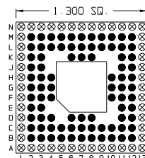
85 Pins – Footprint #13149
