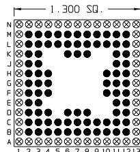
88 Pins – Footprint #13151
