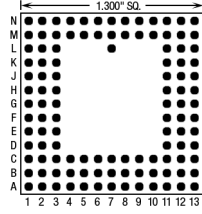
114 Pins – Footprint #13062
