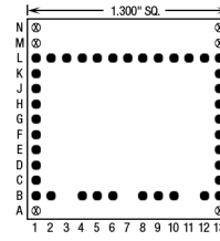
39 Pins – Footprint #13088
