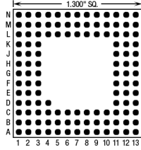
121 Pins – Footprint #13013
