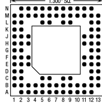
100 Pins – Footprint #13114
