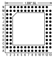
84 Pins – Footprint #13042
