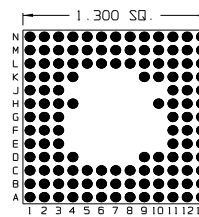
128 Pins – Footprint #13141
