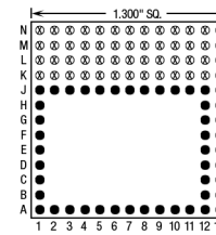
38 Pins – Footprint #13133
