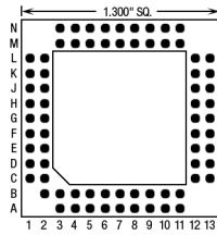
73 Pins – Footprint #13034
