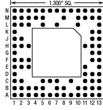
93 Pins – Footprint #13045
