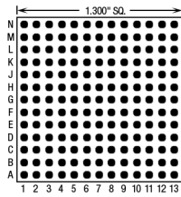
169 Pins – Footprint #13001
