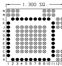
36 Pins – Footprint #13143
