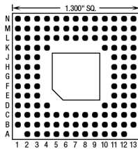
122 Pins – Footprint #13010
