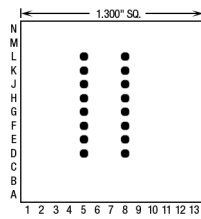
16 Pins – Footprint #13074
