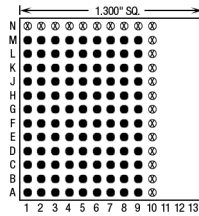
108 Pins – Footprint #13129
