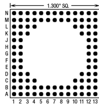
100 Pins – Footprint #13025
