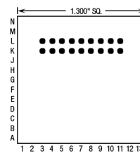
18 Pins – Footprint #13084
