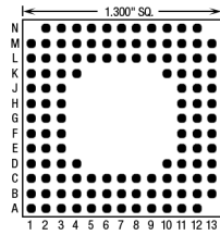
121 Pins – Footprint #13058
