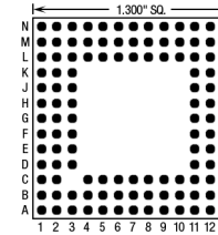
119 Pins – Footprint #13020
