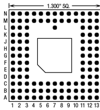
114 Pins – Footprint #13051
