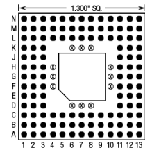
120 Pins – Footprint #13130
