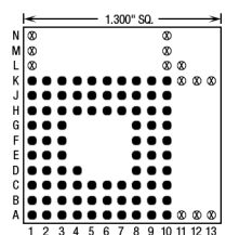
85 Pins – Footprint #13138
