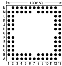
80 Pins – Footprint #13070
