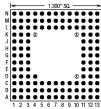
121 Pins – Footprint #13106
