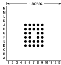
28 Pins – Footprint #13094
