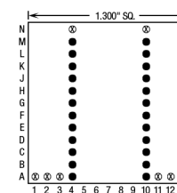
24 Pins – Footprint #13137
