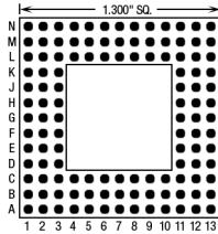
119 Pins – Footprint #13018
