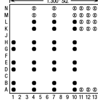
30 Pins – Footprint #13115
