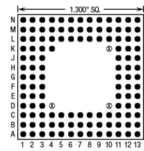
121 Pins – Footprint #13077
