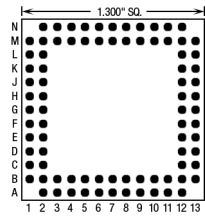
84 Pins – Footprint #13053
