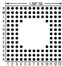
124 Pins – Footprint #13009
