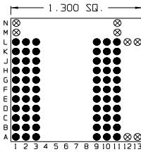
66 Pins – Footprint #13144
