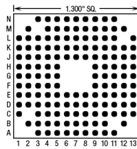
144 Pins – Footprint #13095
