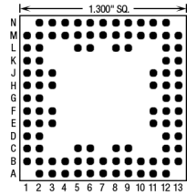
100 Pins – Footprint #13069
