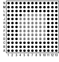
121 Pins – Footprint #13121
