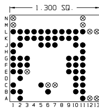
60 Pins – Footprint #13140
