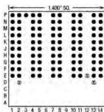
81 Pins – Footprint #14030
