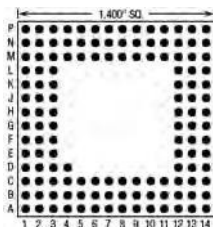
133 Pins – Footprint #14014
