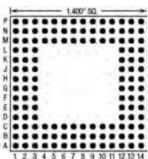
132 Pins – Footprint #14033
