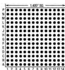
196 Pins – Footprint #14001
