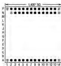
35 Pins – Footprint #14026
