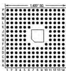
175 Pins – Footprint #14004
