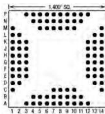
94 Pins – Footprint #14022
