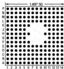
179 Pins – Footprint #14005
