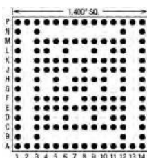
139 Pins – Footprint #14010
