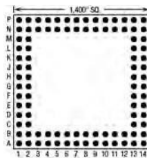
96 Pins – Footprint #14024
