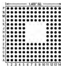
171 Pins – Footprint #14008
