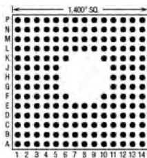
175 Pins – Footprint #14006
