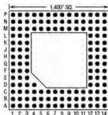
133 Pins – Footprint #14013
