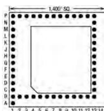
49 Pins – Footprint #14019
