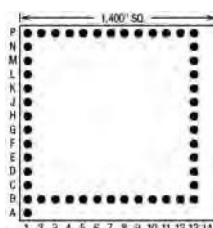
49 Pins – Footprint #14020
