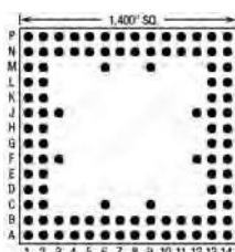
104 Pins – Footprint #14018
