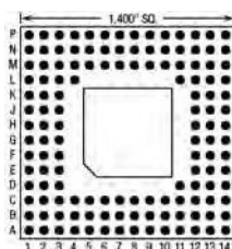
135 Pins – Footprint #14011
