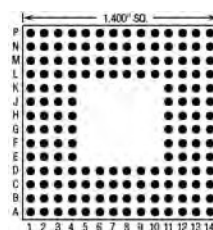
101 Pins – Footprint #14029
