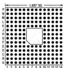
180 Pins – Footprint #14002
