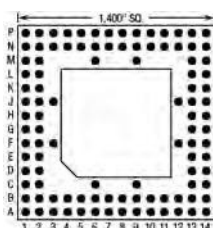
104 Pins – Footprint #14017
