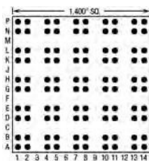
100 Pins – Footprint #14025
