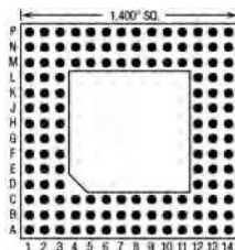
132 Pins – Footprint #14015
