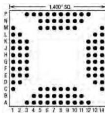
94 Pins – Footprint #14023
