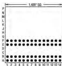
56 Pins – Footprint #14031
