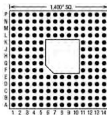
171 Pins – Footprint #14007
