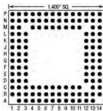
125 Pins – Footprint #14021
