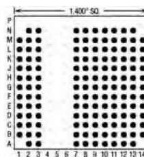
139 Pins – Footprint #14032
