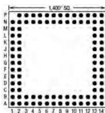
95 Pins – Footprint #14034
