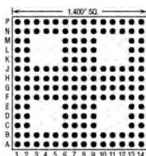
160 Pins – Footprint #14009
