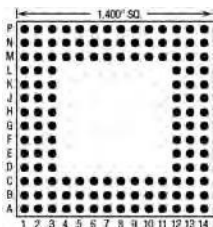
132 Pins – Footprint #14016
