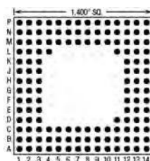
135 Pins – Footprint #14012
