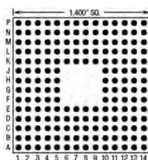
180 Pins – Footprint #14003
