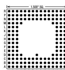
149 Pins – Footprint #15035
