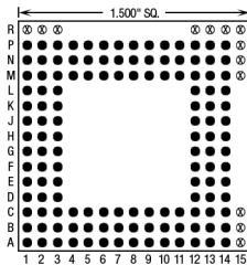
132 Pins – Footprint #15079
