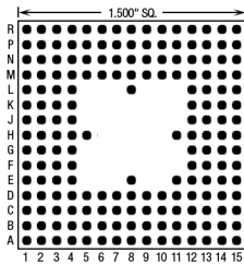
181 Pins – Footprint #15033
