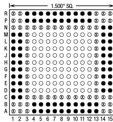
80 Pins – Footprint #15074
