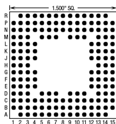
164 Pins – Footprint #15045
