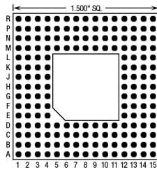
176 Pins – Footprint #15013
