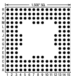
160 Pins – Footprint #15050
