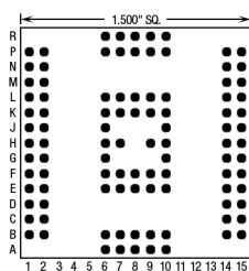
100 Pins – Footprint #15041
