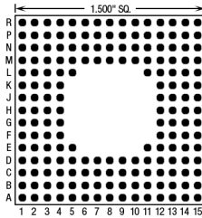
180 Pins – Footprint #15010
