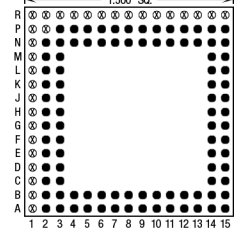
95 Pins – Footprint #15077
