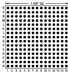
225 Pins – Footprint #15001
