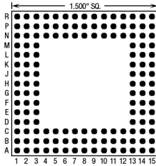
144 Pins – Footprint #15026
