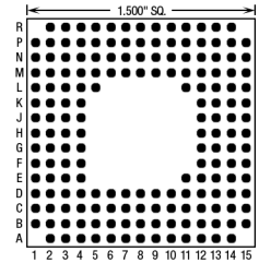
179 Pins – Footprint #15012
