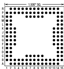
120 Pins – Footprint #15046
