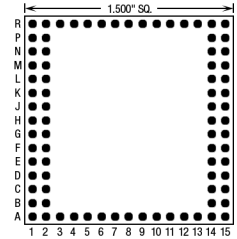
82 Pins – Footprint #15069
