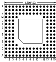
148 Pins – Footprint #15021
