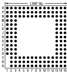
141 Pins – Footprint #15029
