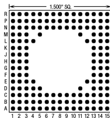
153 Pins – Footprint #15017
