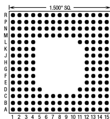
179 Pins – Footprint #15049
