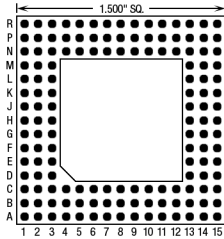
144 Pins – Footprint #15025
