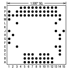
75 Pins – Footprint #15032
