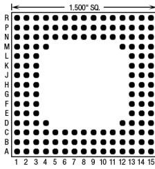
148 Pins – Footprint #15022
