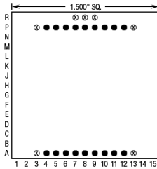
18 Pins – Footprint #15071
