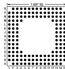
144 Pins – Footprint #15048
