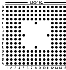
181 Pins – Footprint #15006
