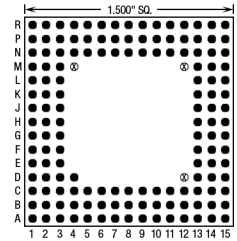
145 Pins – Footprint #15073
