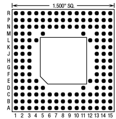
153 Pins – Footprint #15016
