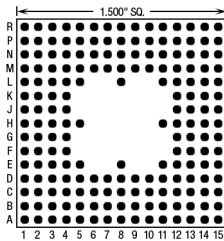
184 Pins – Footprint #15075
