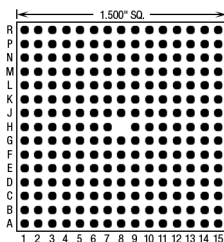
224 Pins – Footprint #15038
