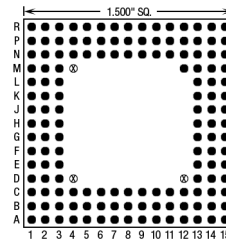
145 Pins – Footprint #15076
