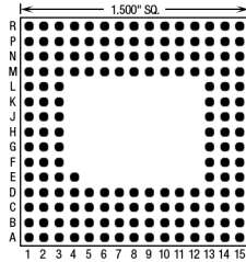
163 Pins – Footprint #15066
