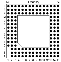
141 Pins – Footprint #15028
