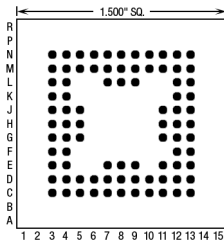
85 Pins – Footprint #15034
