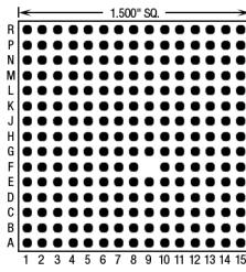
224 Pins – Footprint #15002
