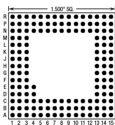
146 Pins – Footprint #15042
