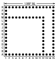
77 Pins – Footprint #15037
