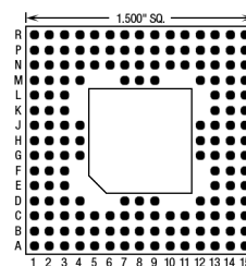
160 Pins – Footprint #15056
