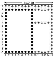
42 Pins – Footprint #15063
