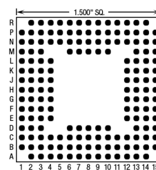
160 Pins – Footprint #15043
