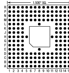
180 Pins – Footprint #15007
