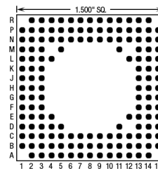
149 Pins – Footprint #15019
