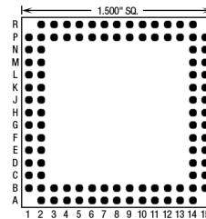
100 Pins – Footprint #15031
