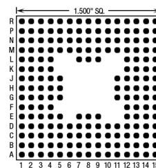
189 Pins – Footprint #15051
