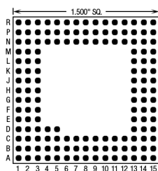
146 Pins – Footprint #15053
