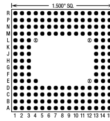
163 Pins – Footprint #15064
