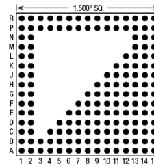
160 Pins – Footprint #15015
