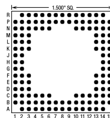
128 Pins – Footprint #15047
