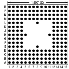
180 Pins – Footprint #15008
