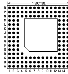
145 Pins – Footprint #15023
