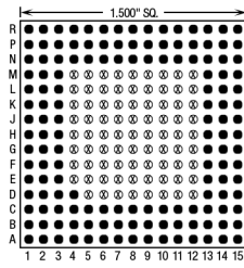
145 Pins – Footprint #15062
