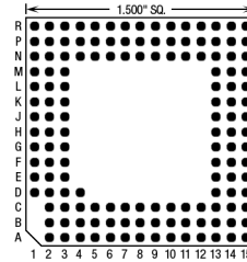
142 Pins – Footprint #15027
