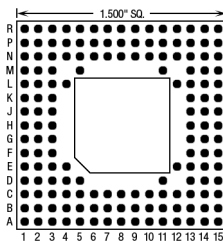
149 Pins – Footprint #15018
