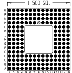
175 Pins – Footprint #15081
