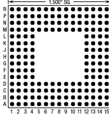
176 Pins – Footprint #15014
