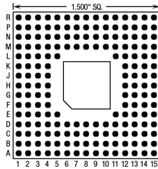
180 Pins – Footprint #15009
