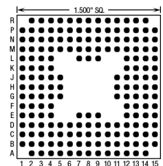
184 Pins – Footprint #15040
