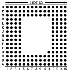
163 Pins – Footprint #15067
