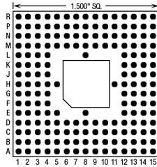
181 Pins – Footprint #15005
