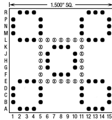
60 Pins – Footprint #15070
