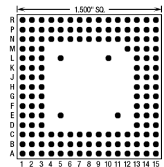
149 Pins – Footprint #15020
