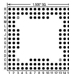
125 Pins – Footprint #15039
