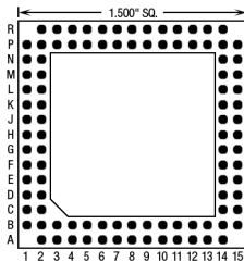
100 Pins – Footprint #15030
