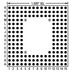
163 Pins – Footprint #15065
