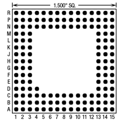
145 Pins – Footprint #15024
