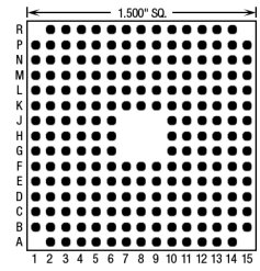
212 Pins – Footprint #15004
