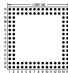
104 Pins – Footprint #15052
