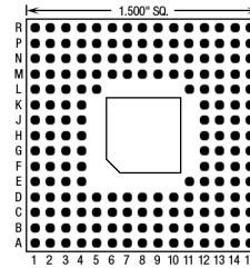
179 Pins – Footprint #15011
