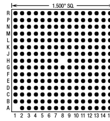
223 Pins – Footprint #15003
