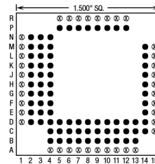
77 Pins – Footprint #15080
