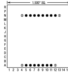
15 Pins – Footprint #15068
