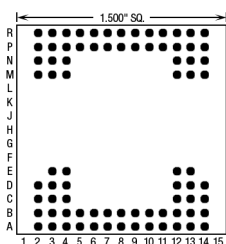
100 Pins – Footprint #15055
