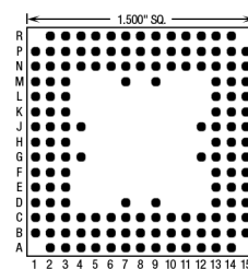
148 Pins – Footprint #15044
