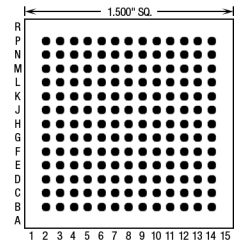
169 Pins – Footprint #15036
