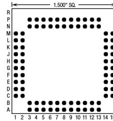
82 Pins – Footprint #15072
