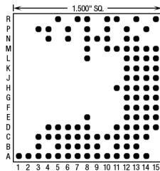
104 Pins – Footprint #15078
