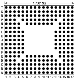
54 Pins – Footprint #17035
