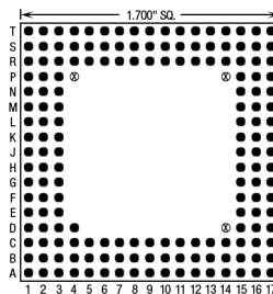
169 Pins – Footprint #17053
