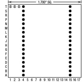
240 Pins – Footprint #17033
