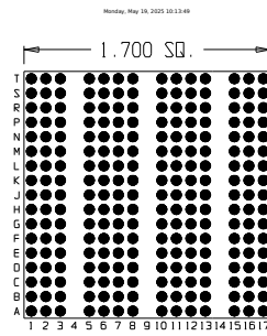
238 Pins – Footprint #17064
