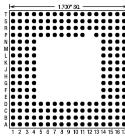
207 Pins – Footprint #17045
