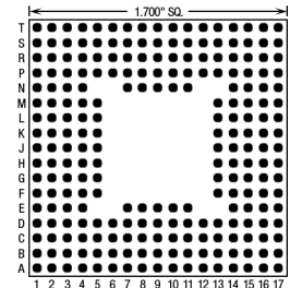
232 Pins – Footprint #17037
