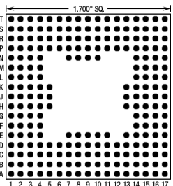
226 Pins – Footprint #17060
