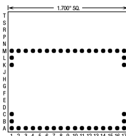
43 Pins – Footprint #17014
