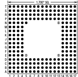
209 Pins – Footprint #17029
