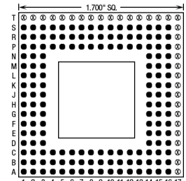
156 Pins – Footprint #17050
