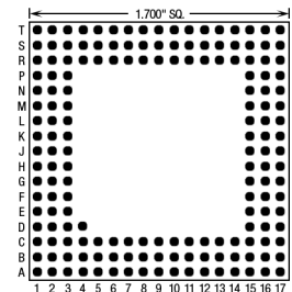
169 Pins – Footprint #17012
