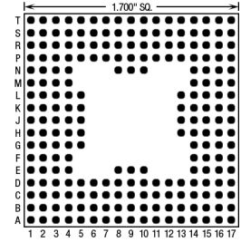
225 Pins – Footprint #17008
