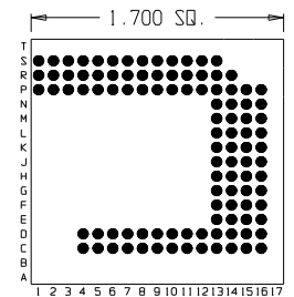
105 Pins – Footprint #17054
