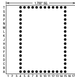
34 Pins – Footprint #17034
