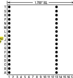
34 Pins – Footprint #17028
