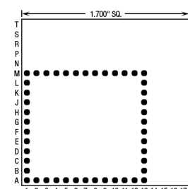
54 Pins – Footprint #17058
