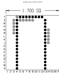
40 Pins – Footprint #17063
