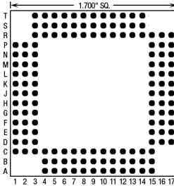
144 Pins – Footprint #17006
