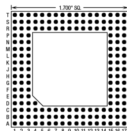
169 Pins – Footprint #17013
