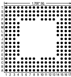
196 Pins – Footprint #17022
