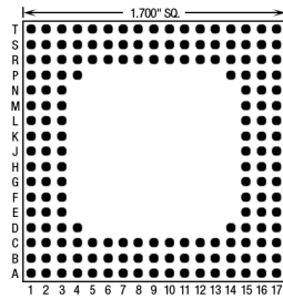
172 Pins – Footprint #17021
