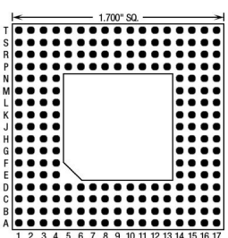
208 Pins – Footprint #17059
