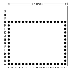
54 Pins – Footprint #17016
