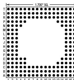
181 Pins – Footprint #17015
