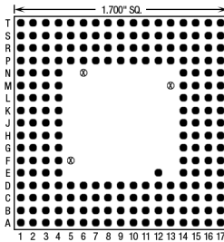
209 Pins – Footprint #17018
