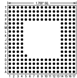
209 Pins – Footprint #17020
