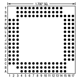
145 Pins – Footprint #17004
