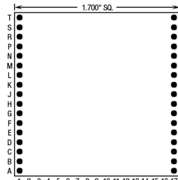
34 Pins – Footprint #17047
