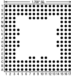
185 Pins – Footprint #17031
