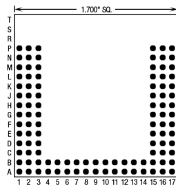
106 Pins – Footprint #17051
