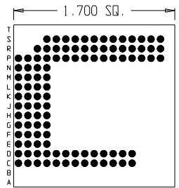
105 Pins – Footprint #17055
