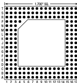
169 Pins – Footprint #17010
