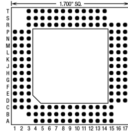
144 Pins – Footprint #17005
