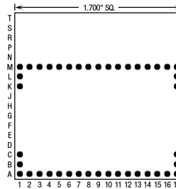
43 Pins – Footprint #17019
