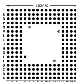
209 Pins – Footprint #17057
