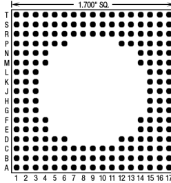
188 Pins – Footprint #17032
