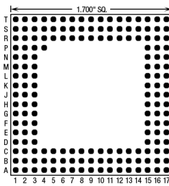
169 Pins – Footprint #17002
