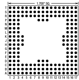
180 Pins – Footprint #17024
