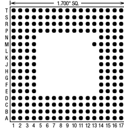
209 Pins – Footprint #17030
