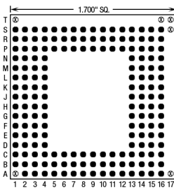
175 Pins – Footprint #17044
