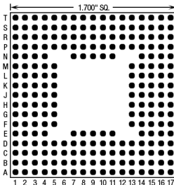
228 Pins – Footprint #17036
