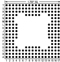
192 Pins – Footprint #17025
