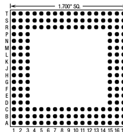
168 Pins – Footprint #17011
