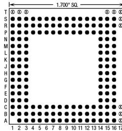
155 Pins – Footprint #17061
