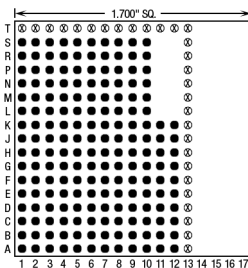
180 Pins – Footprint #17052
