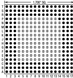
169 Pins – Footprint #17026
