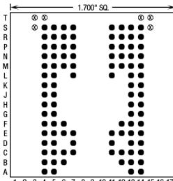
100 Pins – Footprint #17048
