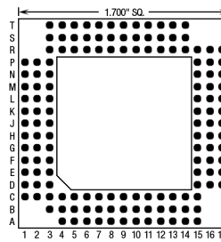
145 Pins – Footprint #17003
