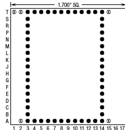
54 Pins – Footprint #17038
