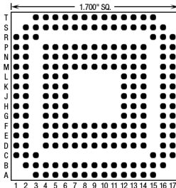
208 Pins – Footprint #17039
