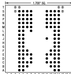
100 Pins – Footprint #17049
