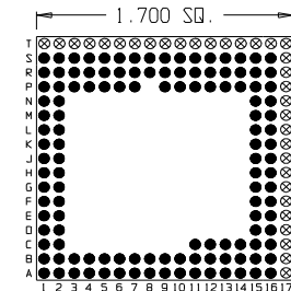
127 Pins – Footprint #17062
