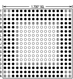
104 Pins – Footprint #17056
