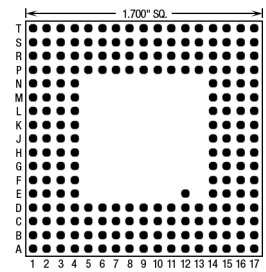
209 Pins – Footprint #17046
