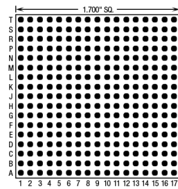
289 Pins – Footprint #17001
