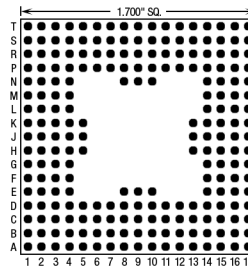
216 Pins – Footprint #17023
