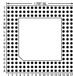
168 Pins – Footprint #17009
