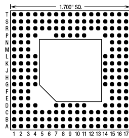
192 Pins – Footprint #17043
