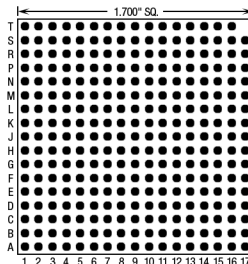
288 Pins – Footprint #17040
