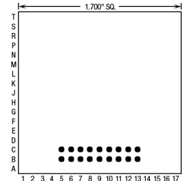
18 Pins – Footprint #17041
