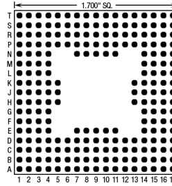
225 Pins – Footprint #17007
