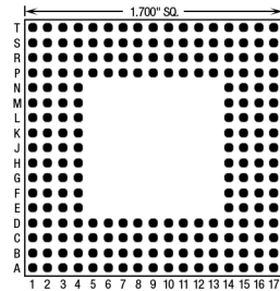
208 Pins – Footprint #17017
