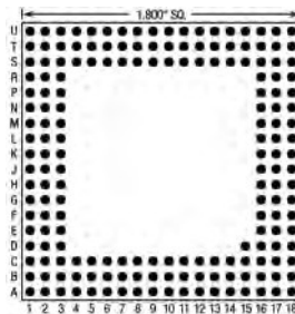
181 Pins – Footprint #18040
