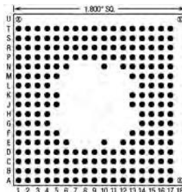
242 Pins – Footprint #18036
