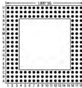
180 Pins – Footprint #18006
