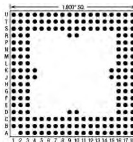
191 Pins – Footprint #18015
