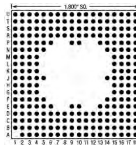
241 Pins – Footprint #18028
