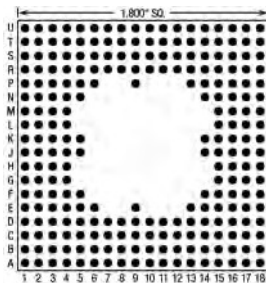
242 Pins – Footprint #18026
