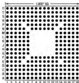
281 Pins – Footprint #18035
