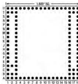
106 Pins – Footprint #18019
