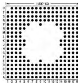
241 Pins – Footprint #18027
