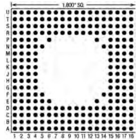
233 Pins – Footprint #18008
