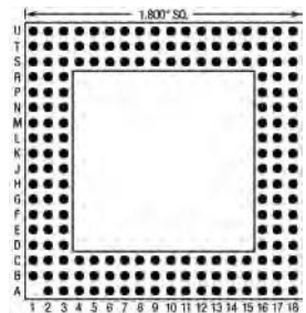
179 Pins – Footprint #18020
