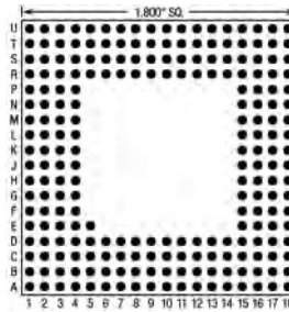
225 Pins – Footprint #18003
