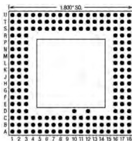
182 Pins – Footprint #18022
