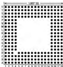
223 Pins – Footprint #18013
