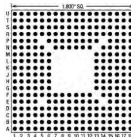
281 Pins – Footprint #18037
