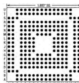
240 Pins – Footprint #18033
