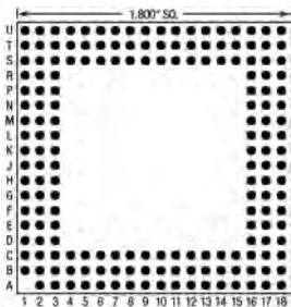
179 Pins – Footprint #18038
