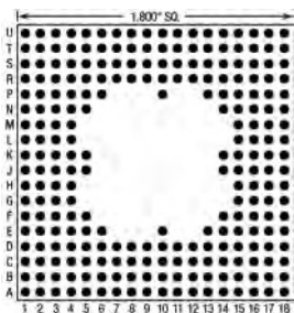
241 Pins – Footprint #18021
