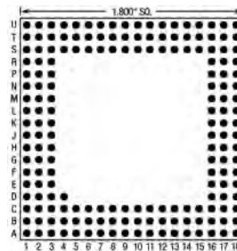
181 Pins – Footprint #18041
