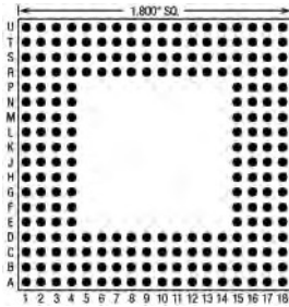
224 Pins – Footprint #18005
