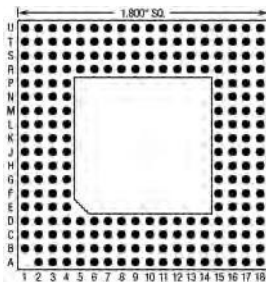
223 Pins – Footprint #18039
