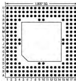
191 Pins – Footprint #18018
