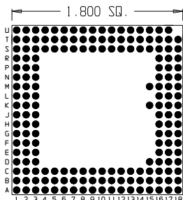
182 Pins – Footprint #18043
