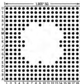
246 Pins – Footprint #18034
