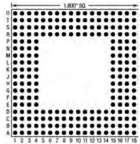
224 Pins – Footprint #18012
