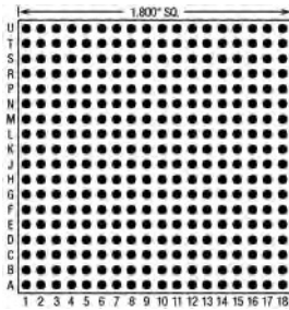
324 Pins – Footprint #18001
