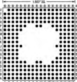
241 Pins – Footprint #18025-ZIF
