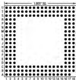
179 Pins – Footprint #18030
