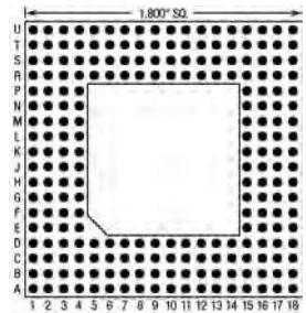
224 Pins – Footprint #18004
