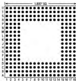
223 Pins – Footprint #18017
