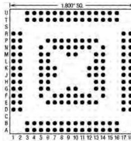
160 Pins – Footprint #18011
