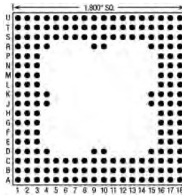
192 Pins – Footprint #18010
