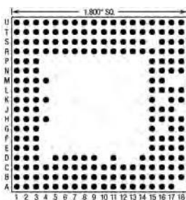
206 Pins – Footprint #18042
