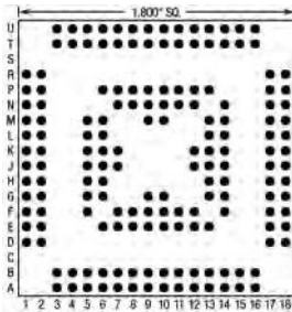
159 Pins – Footprint #18009
