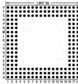
180 Pins – Footprint #18007
