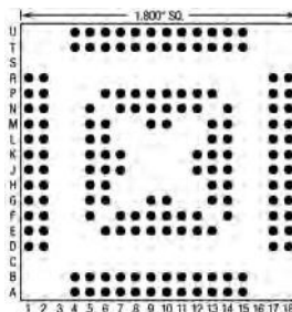
160 Pins – Footprint #18014
