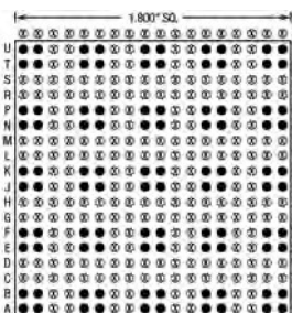
100 Pins – Footprint #18023-ZIP
