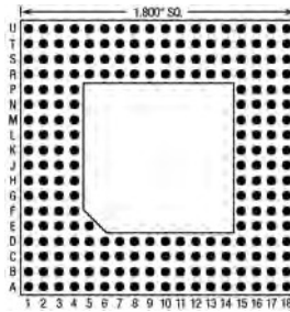
225 Pins – Footprint #18002
