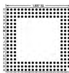
179 Pins – Footprint #18024
