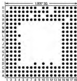
206 Pins – Footprint #18031
