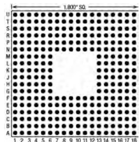
288 Pins – Footprint #18016
