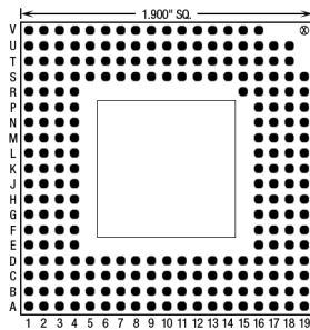
236 Pins – Footprint #19009
