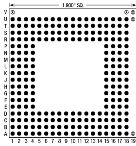
224 Pins – Footprint #19044
