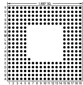
281 Pins – Footprint #19010
