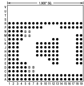
161 Pins – Footprint #19037
