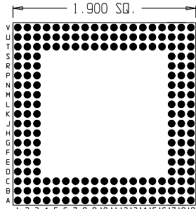
192 Pins – Footprint #19051
