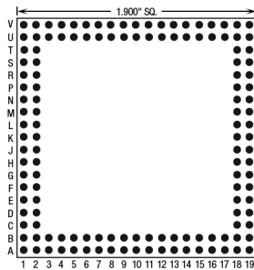
136 Pins – Footprint #19008
