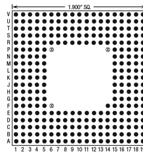
281 Pins – Footprint #19028
