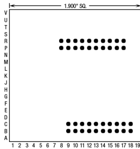
40 Pins – Footprint #19042
