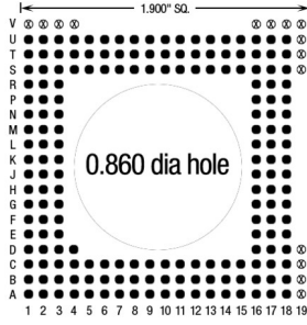
181 Pins – Footprint #19048
