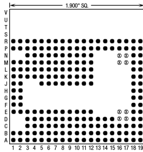
200 Pins – Footprint #19036
