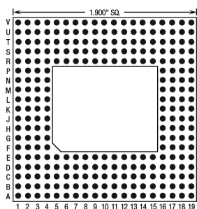
262 Pins – Footprint #19014
