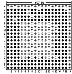
206 Pins – Footprint #19046
