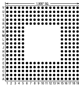
280 Pins – Footprint #19006
