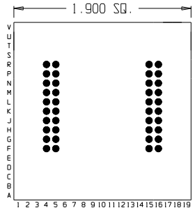
40 Pins – Footprint #19050
