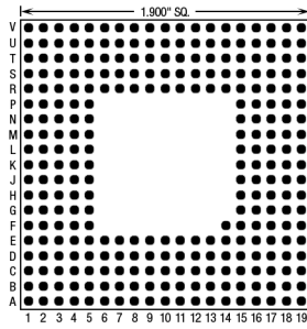
281 Pins – Footprint #19045
