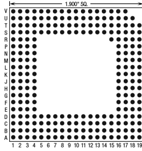
238 Pins – Footprint #19007
