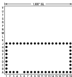
51 Pins – Footprint #19018
