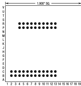
44 Pins – Footprint #19041
