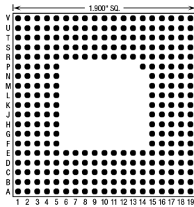
281 Pins – Footprint #19012
