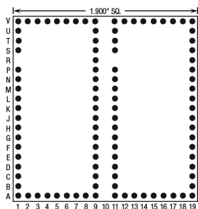
102 Pins – Footprint #19017
