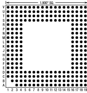
238 Pins – Footprint #19004
