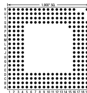
237 Pins – Footprint #19019
