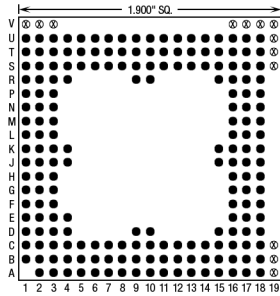
191 Pins – Footprint #19047
