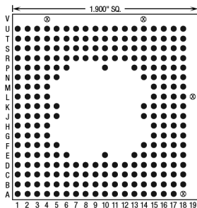
241 Pins – Footprint #19021
