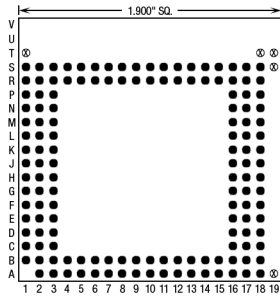
143 Pins – Footprint #19035
