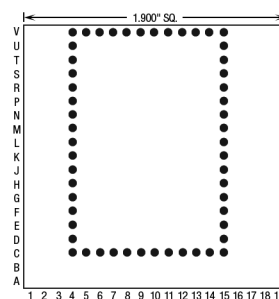
54 Pins – Footprint #19016
