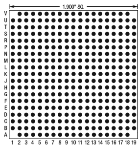
357 Pins – Footprint #19026
