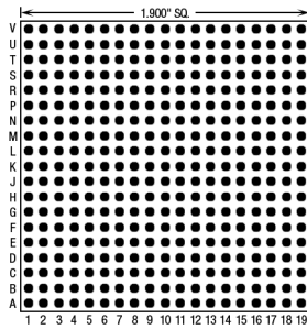
361 Pins – Footprint #19001
