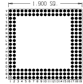
106 Pins – Footprint #19049
