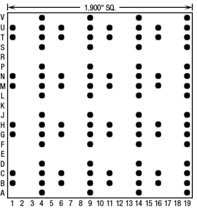
96 Pins – Footprint #19038
