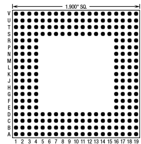
240 Pins – Footprint #19013
