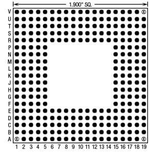
277 Pins – Footprint #19005
