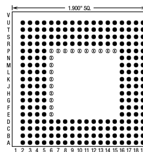
224 Pins – Footprint #19025
