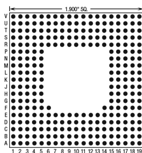
282 Pins – Footprint #19030
