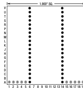
39 Pins – Footprint #19022
