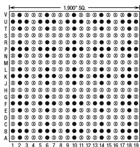
125 Pins – Footprint #19023
