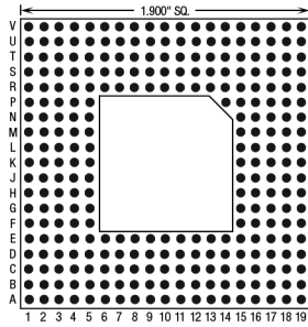
281 Pins – Footprint #19032
