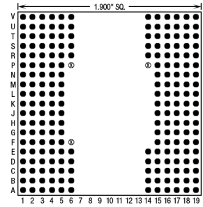
210 Pins – Footprint #19034
