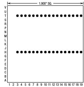
34 Pins – Footprint #19003
