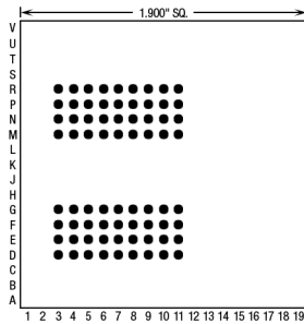
72 Pins – Footprint #19011
