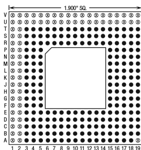
280 Pins – Footprint #19024
