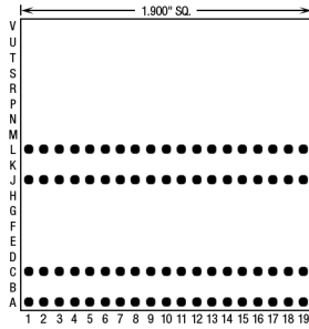
76 Pins – Footprint #19033
