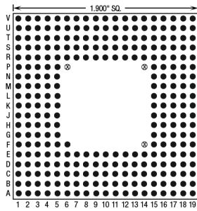
281 Pins – Footprint #19029
