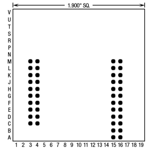
44 Pins – Footprint #19040
