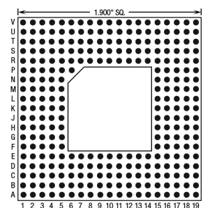
281 Pins – Footprint #19031
