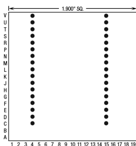
34 Pins – Footprint #19015
