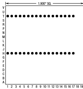
34 Pins – Footprint #19002
