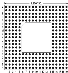
280 Pins – Footprint #19027
