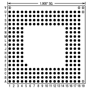
225 Pins – Footprint #19043
