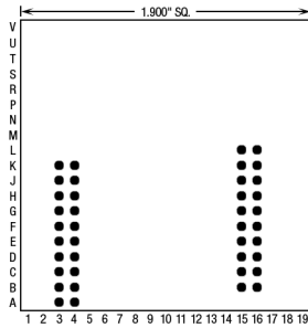
40 Pins – Footprint #19039
