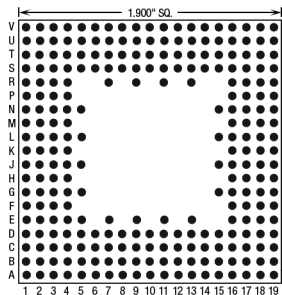
257 Pins – Footprint #19020
