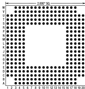
240 Pins – Footprint #20010
