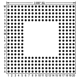
299 Pins – Footprint #20009
