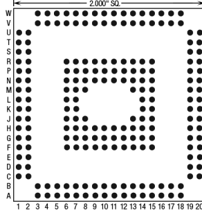
208 Pins – Footprint #20008
