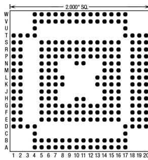
240 Pins – Footprint #20014
