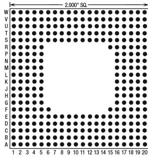
303 Pins – Footprint #20004
