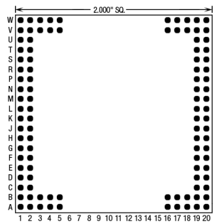
104 Pins – Footprint #20021
