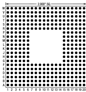
336 Pins – Footprint #20019
