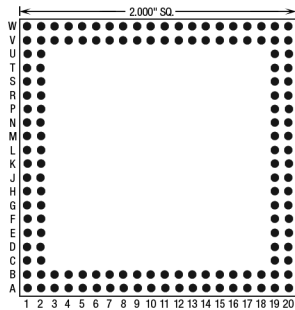
144 Pins – Footprint #20007
