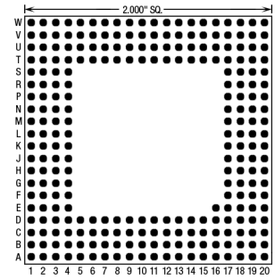
257 Pins – Footprint #20018
