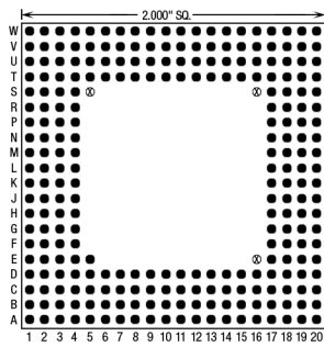
257 Pins – Footprint #20013
