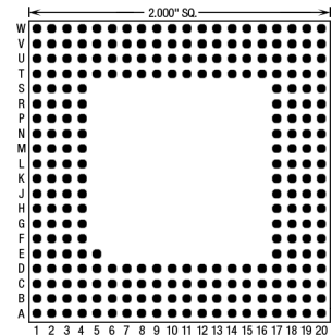
257 Pins – Footprint #20012
