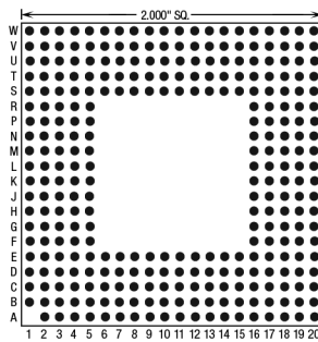
299 Pins – Footprint #20002
