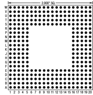
300 Pins – Footprint #20006
