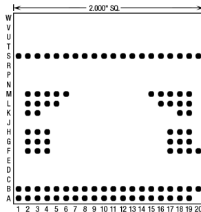
100 Pins – Footprint #20011
