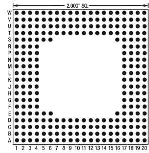
262 Pins – Footprint #20003
