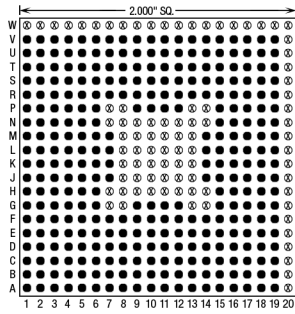
352 Pins (393?) – Footprint #20016
