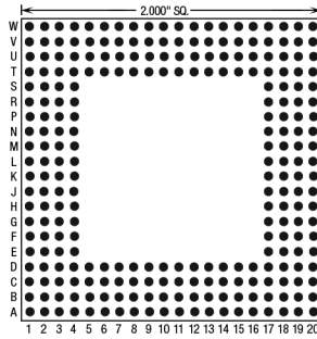
256 Pins – Footprint #20005
