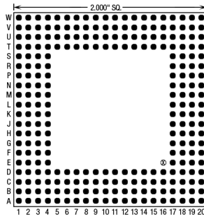
256 Pins – Footprint #20017
