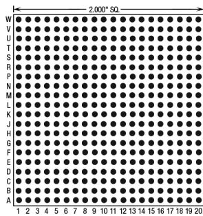
400 Pins – Footprint #20001
