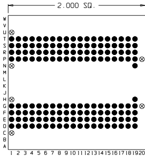
162 Pins – Footprint #20020
