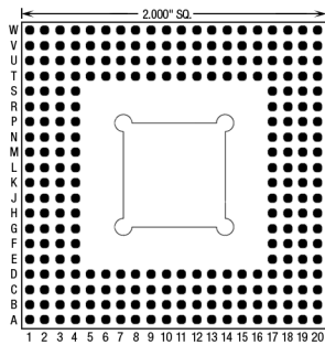
256 Pins – Footprint #20022
