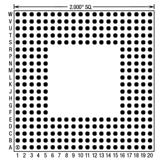
299 Pins – Footprint #20015
