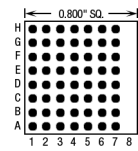
56 Pins – Footprint #08004
