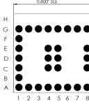
30 Pins – Footprint #08006
