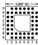
44 Pins – Footprint #08002
