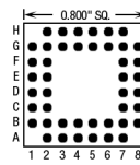
44 Pins – Footprint #08003
