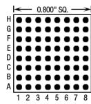
64 Pins – Footprint #08001
