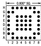
44 Pins – Footprint #08005
