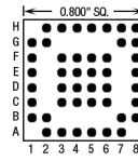
45 Pins – Footprint #08007
