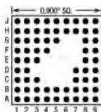
65 Pins – Footprint #09006
