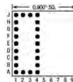
22 Pins – Footprint #09028
