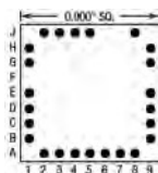
24 Pins – Footprint #09023
