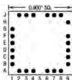
24 Pins – Footprint #09022
