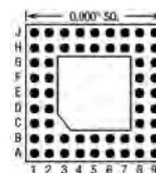
56 Pins – Footprint #09008
