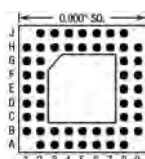
52 Pins – Footprint #09019
