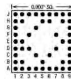
49 Pins – Footprint #09012
