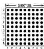
81 Pins – Footprint #09001
