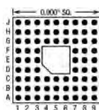
72 Pins – Footprint #09003
