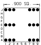
18 Pins – Footprint #09026
