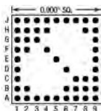
49 Pins – Footprint #09014
