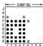
28 Pins – Footprint #09029
