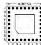
32 Pins – Footprint #09016
