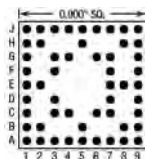
53 Pins – Footprint #09011
