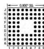
72 Pins – Footprint #09004
