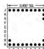
22 Pins – Footprint #09020
