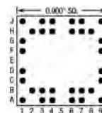
32 Pins – Footprint #09024
