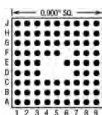
75 Pins – Footprint #09002
