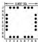
22 Pins – Footprint #09025
