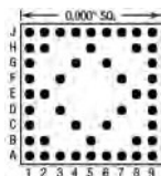
48 Pins – Footprint #09013
