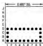
22 Pins – Footprint #09021
