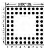
56 Pins – Footprint #09009
