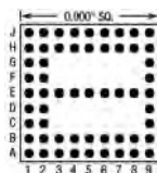
57 Pins – Footprint #09007
