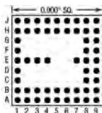
55 Pins – Footprint #09010
