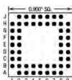
52 Pins – Footprint #09018
