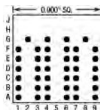
40 Pins – Footprint #09015
