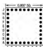
32 Pins – Footprint #09017
